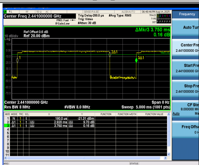
2DHS_Ant1_2441
