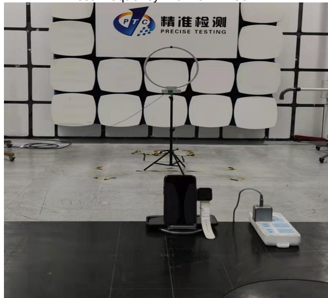
Radiated Spurious Emissions Test Frequency From 9KHz-30MHz
