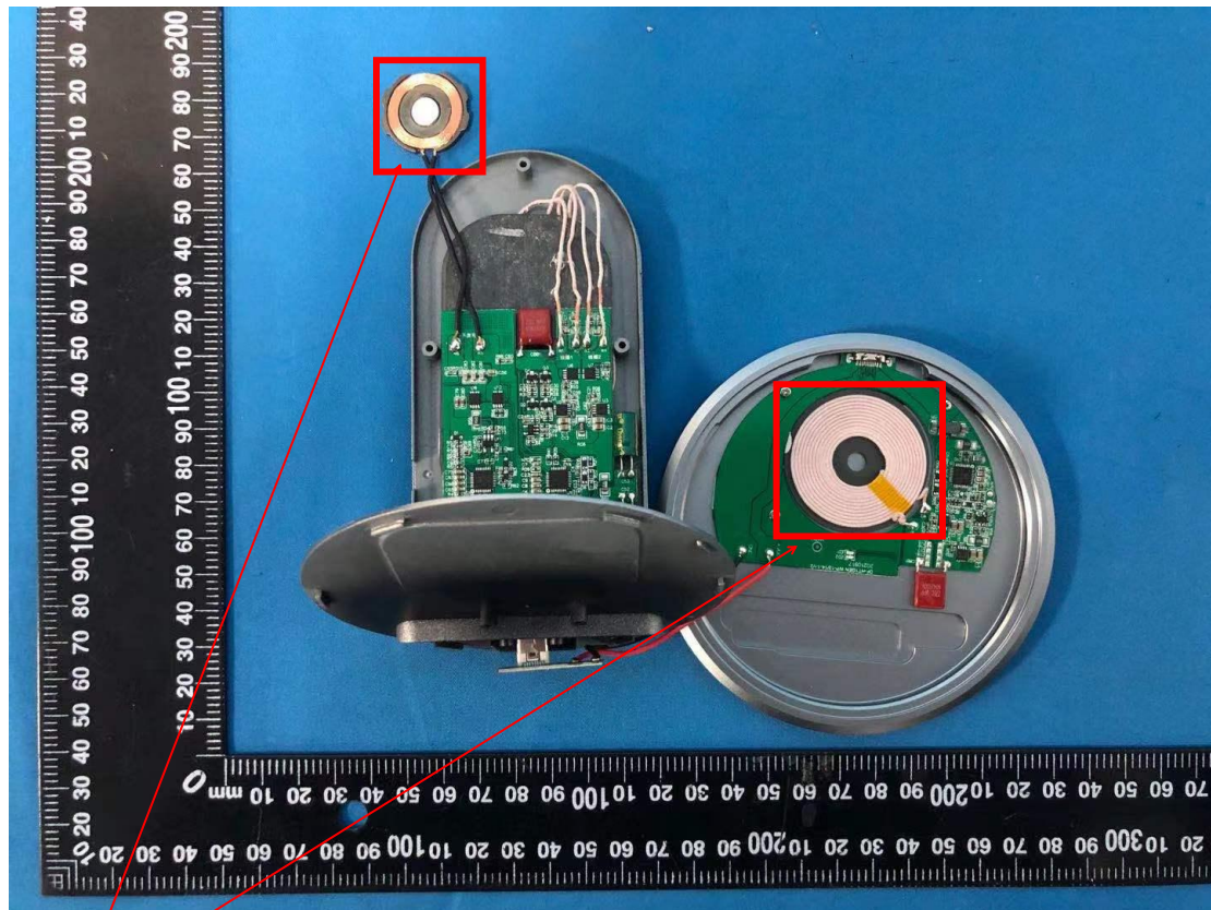
Coil ANT
