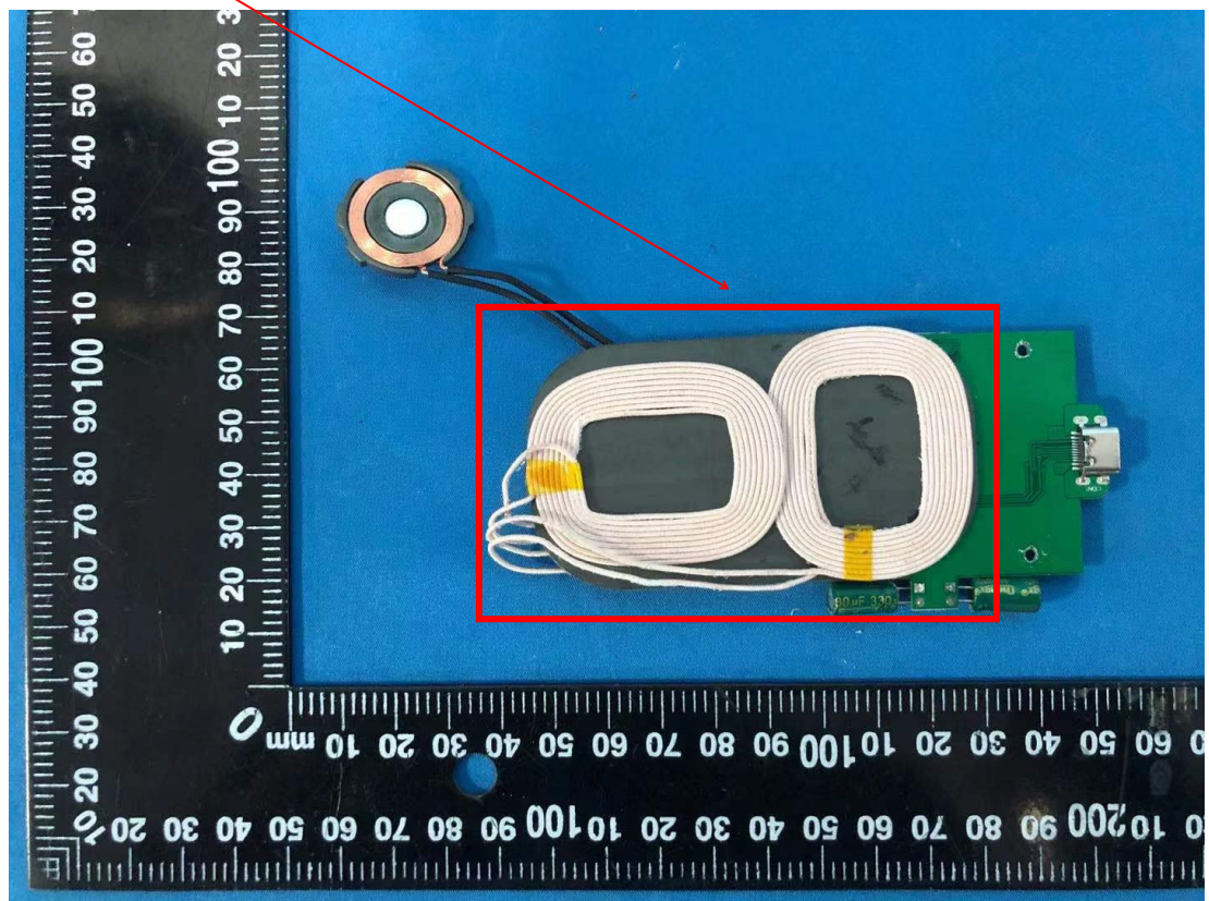
Coil ANT
