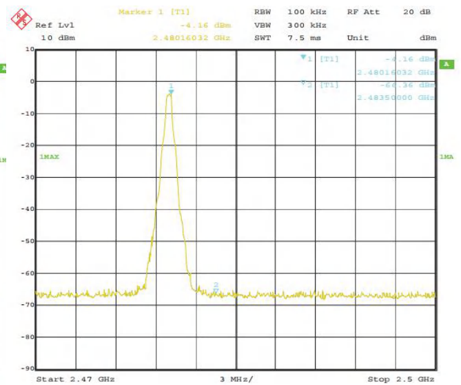
GFSK: Band Edge-High Channel
