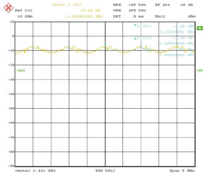
( \pi /4DQPSK) Channel Separation plot
