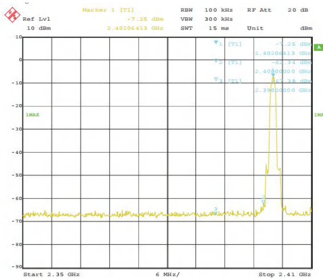
\pi/4 -DQPSK: Band Edge-Low Channel
