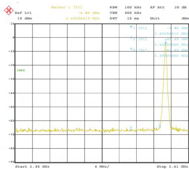
GFSK: Band Edge-Low Channel
