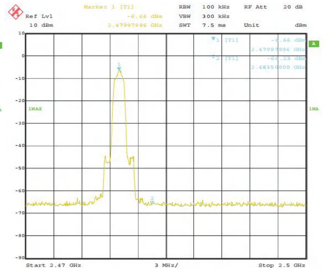
\pi/4 -DQPSK: Band Edge-High Channel
