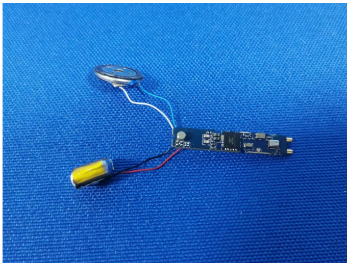
Ceramic Antenna
