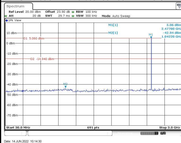
CSE Plot on CH 78 between 30 MHz ~ 3 GHz
