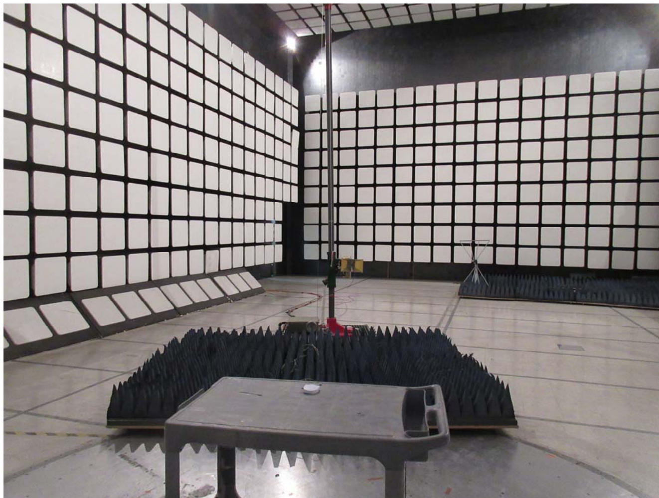
Radiated Emissions at 3 m (Above 1 GHz) Orthogonal Position 1
