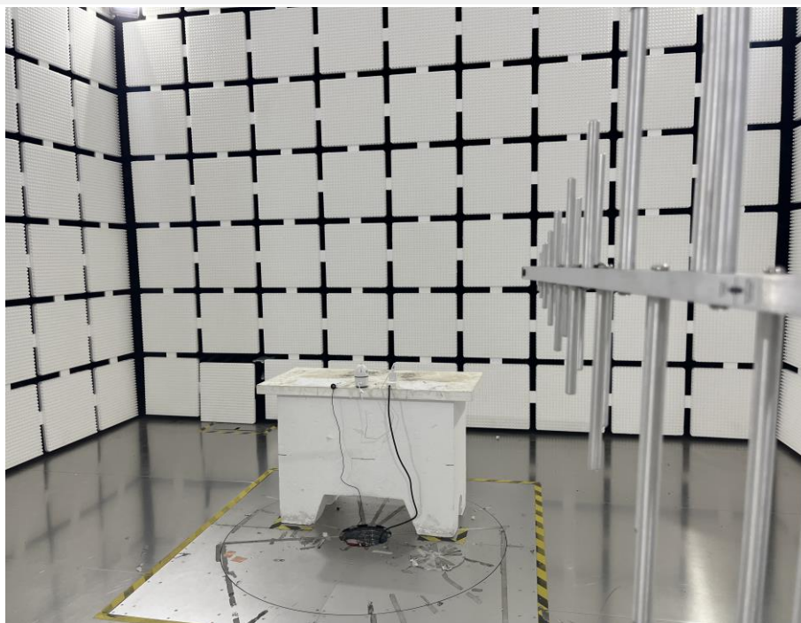
RSE-30MHz-1GHz
