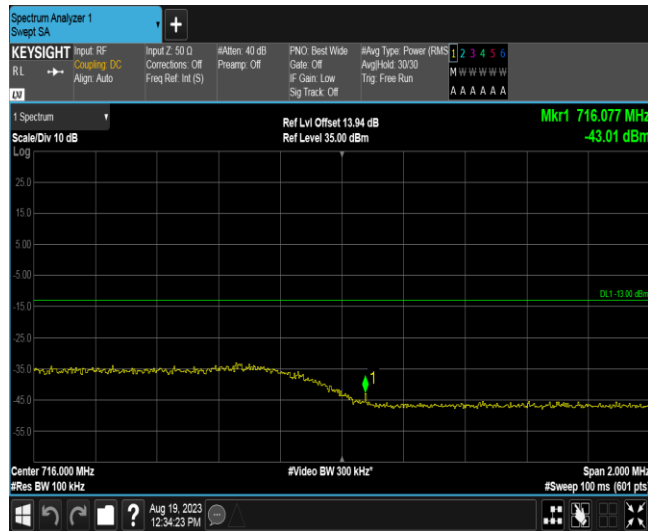
Band12-5MHz-16QAM-23155-1RB#24
