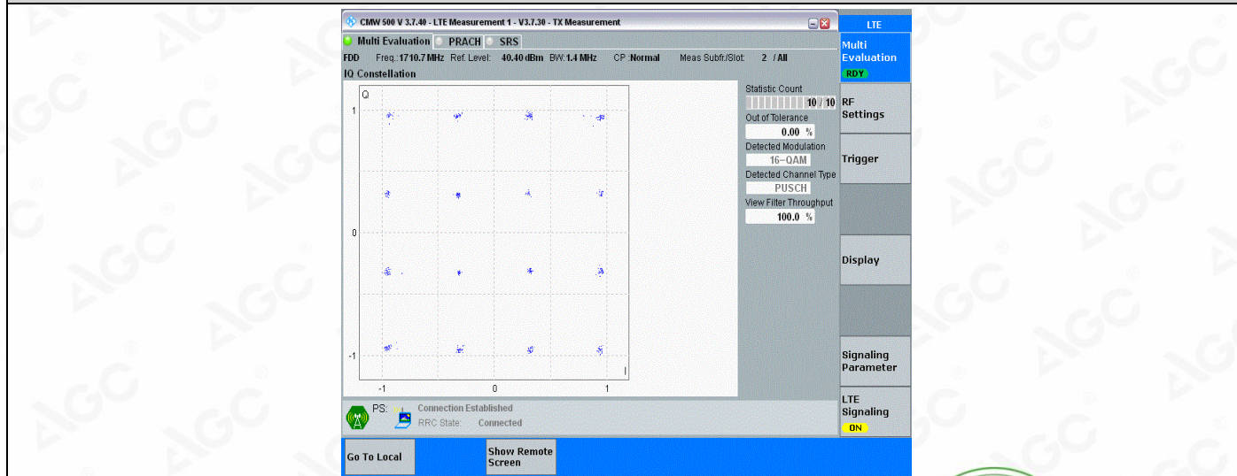
Band4-1.4MHz-16QAM-20175-6RB#0
