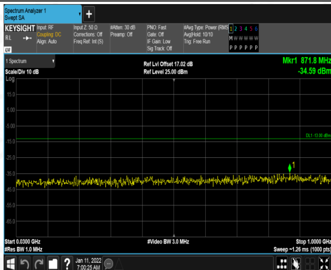
Band4-5MHz-QPSK-19975-1RB#0-Range1:30~1000MHz
