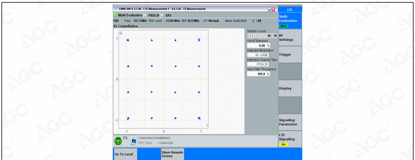
Band12-10MHz-16QAM-23130-50RB#0
