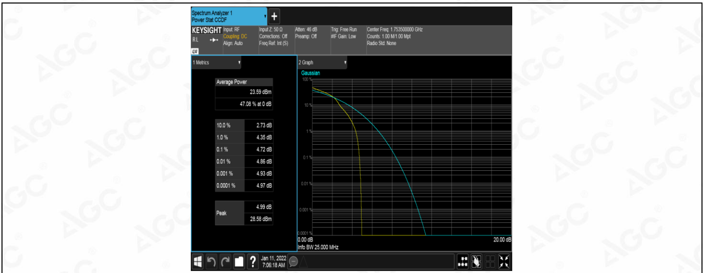
Band4-3MHz-16QAM-20385-15RB#0
