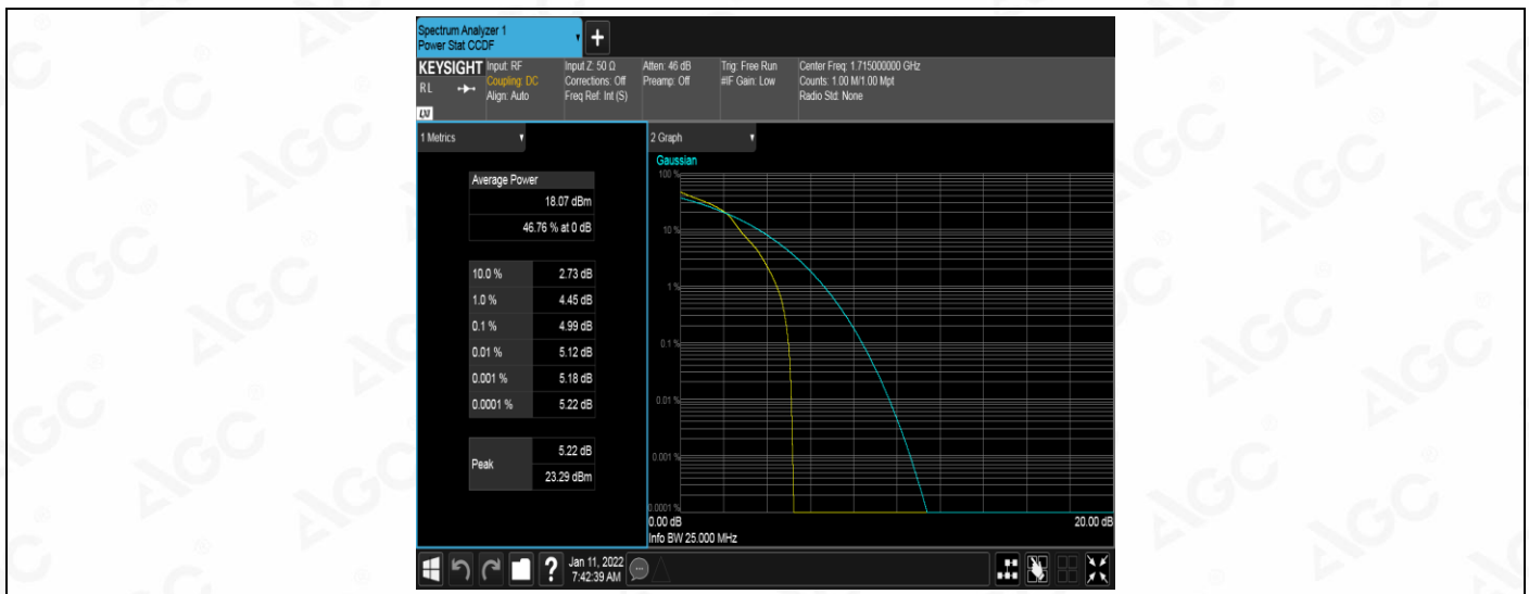
Band4-10MHz-16QAM-20000-50RB#0
