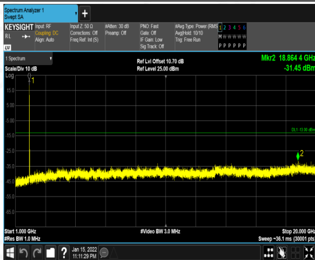
Band2-15MHz-16QAM-18900-1RB#0-Range2:1000~20000MHz
