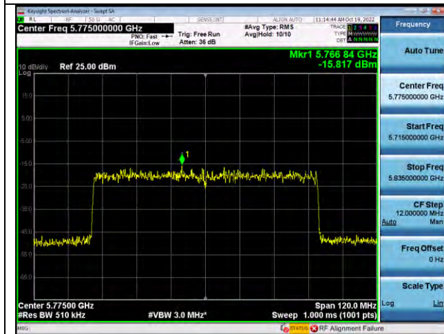
CH155 -5775MHz
