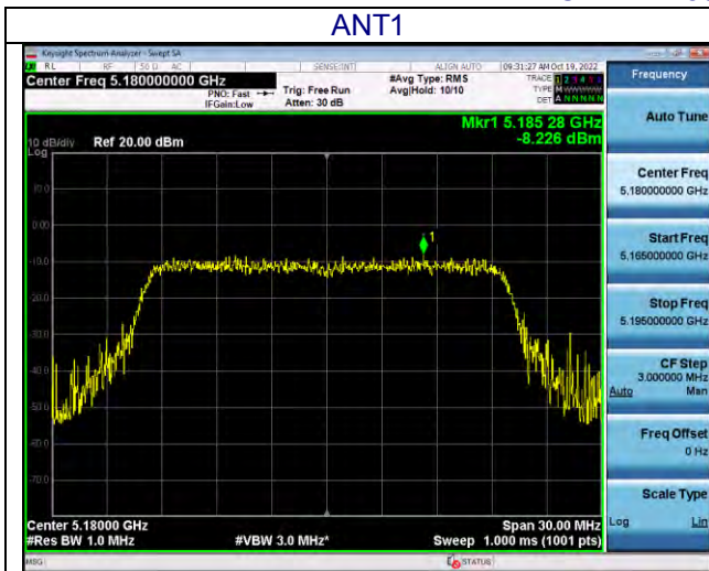
CH36-5180MHz
