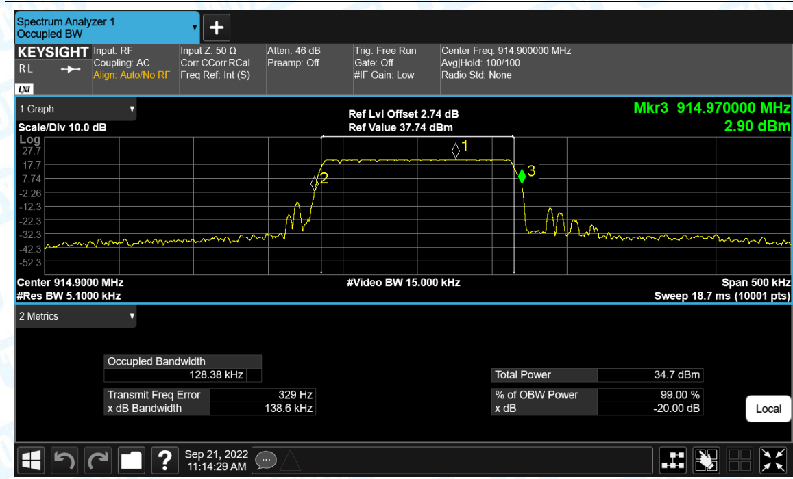
-20dB Bandwidth NVNT user 914.9MHz Ant1
