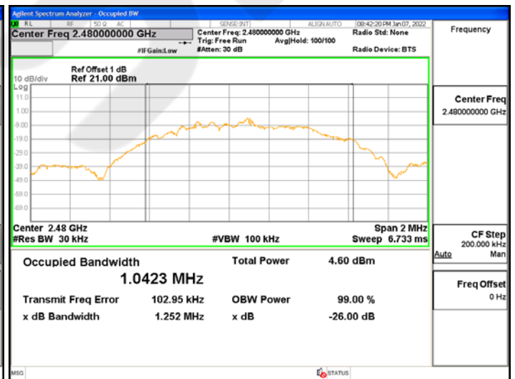
99% Bandwidth Mode3 CH39
