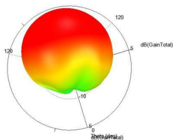
Gain Plot 2
