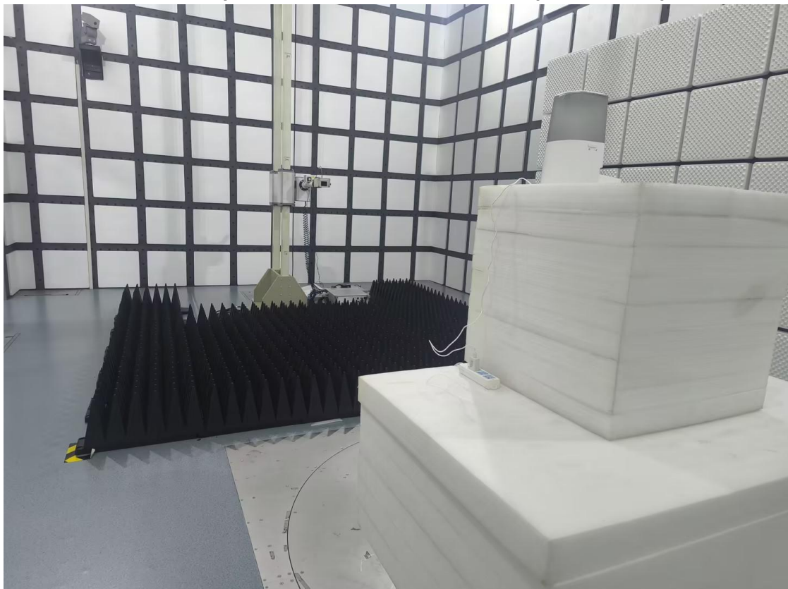
Radiated Spurious Emissions Test Side View (Above 18GHz)
