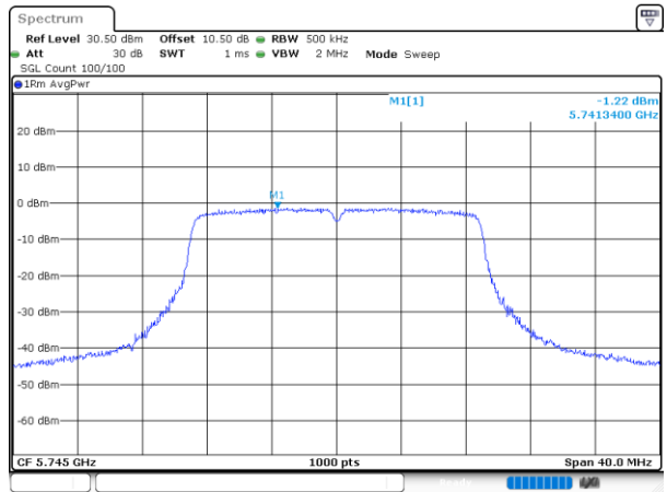
802.11n20_5745MHz
