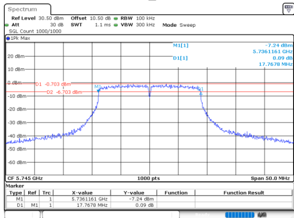
802.11n20_5745MHz
