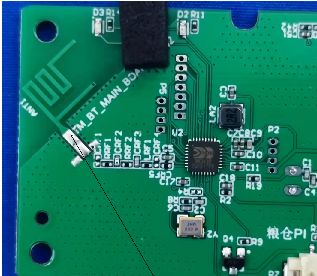
PCB ANTENNA
