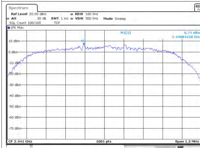
Tx. Spurious NVNT 2-DH5 2441MHz Ref
