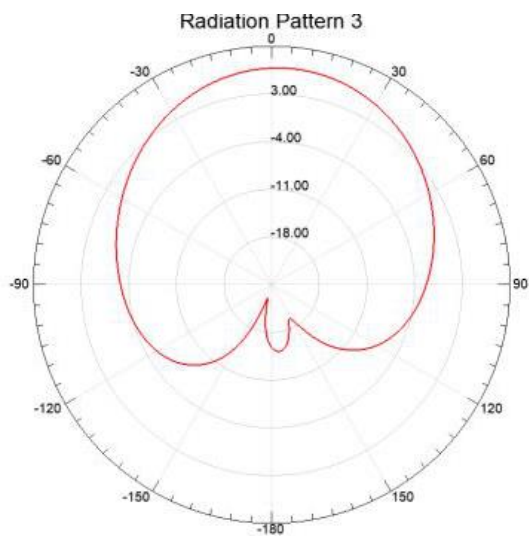
Fig4. \theta = 0^\circ @ 24.1\text{GHz}
