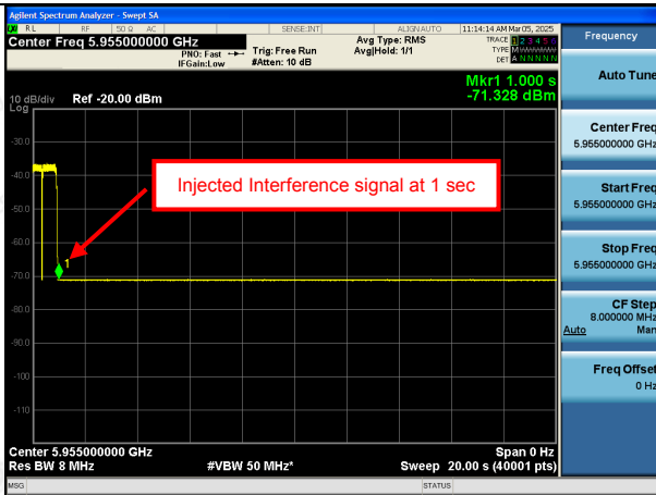
802.11ax (HE160) / CH15 (Middle Edge)
