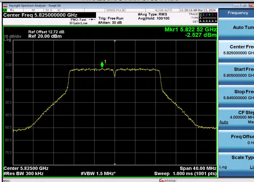
11AX20SISO-Ant1-5825-PASS
