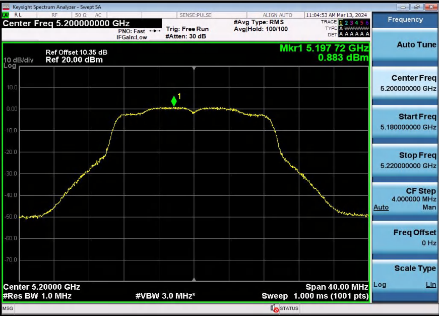
11AX20SISO-Ant1-5200-PASS
