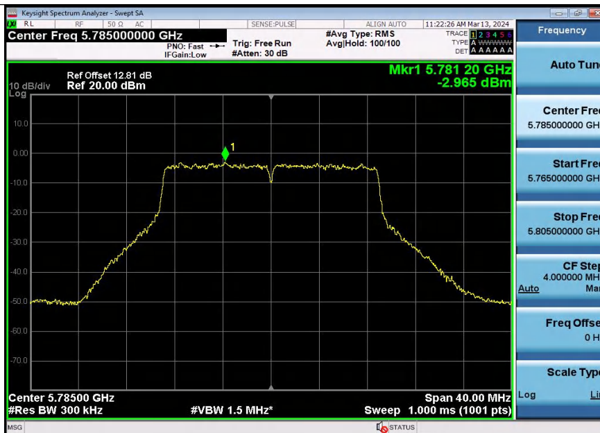
11AX20SISO-Ant1-5785-PASS
