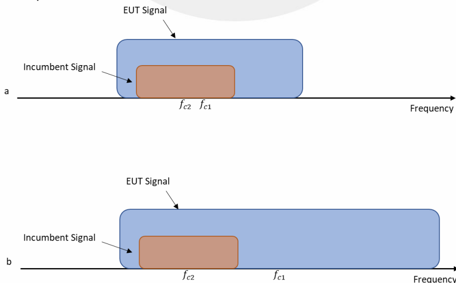
Figure. Two possible scenarios where a) center frequency of EUT transmission falls within incumbent's bandwidth, or b) outside of it
