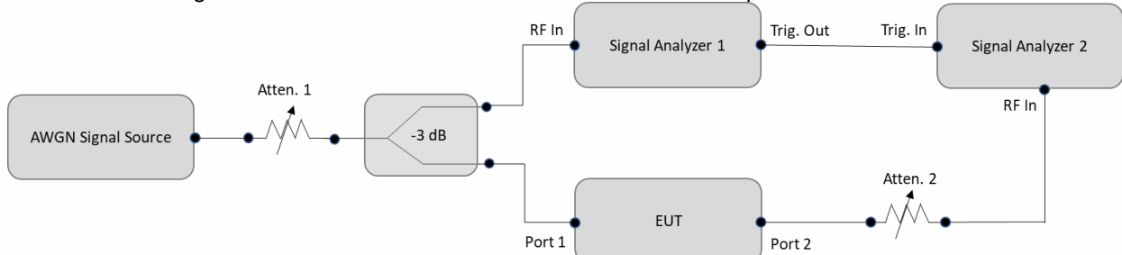
Figure. Contention-based protocol test setup, conducted method Step-by-Step Procedure, Conducted Setup
