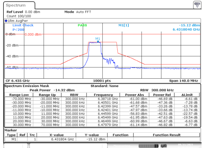
MIMO-B, 802.11ax/be20-MCS0, Ch97-8m-53
