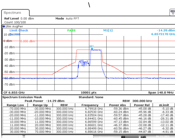
MIMO-A, 802.11ax/be20-MCS0, Ch181-8m-53
