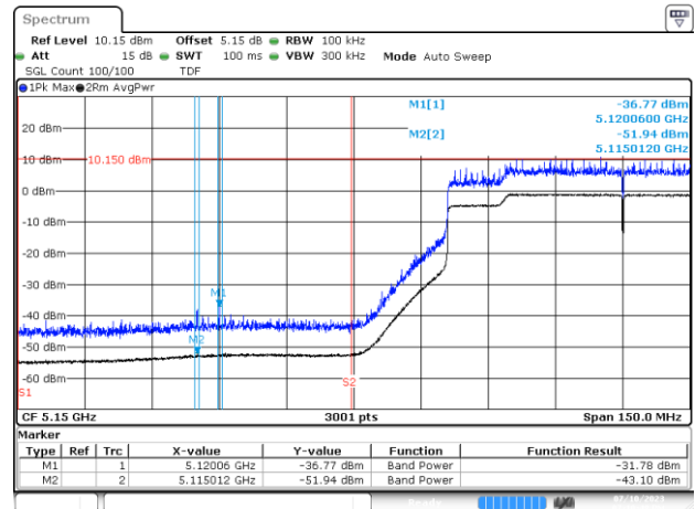
BE-R-LOW, SISO-A, 802.11ax/be80-MCS0, Ch42
