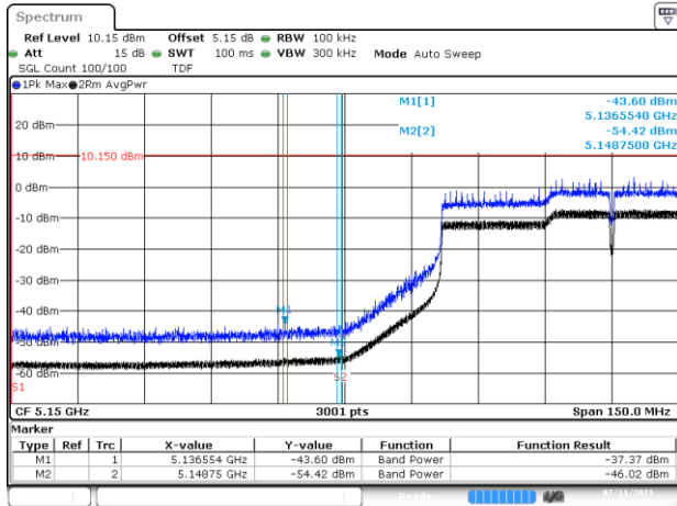
BE-R-LOW, MIMO-A, 802.11ac160-VHT8, Ch50
