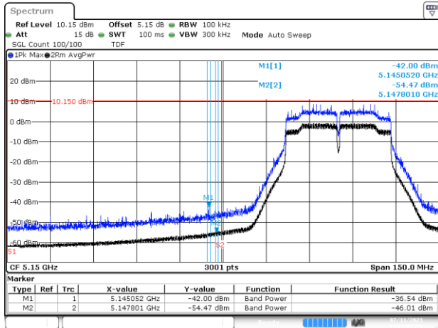
BE-R-LOW, MIMO-A, 802.11n40-HT8, Ch38
