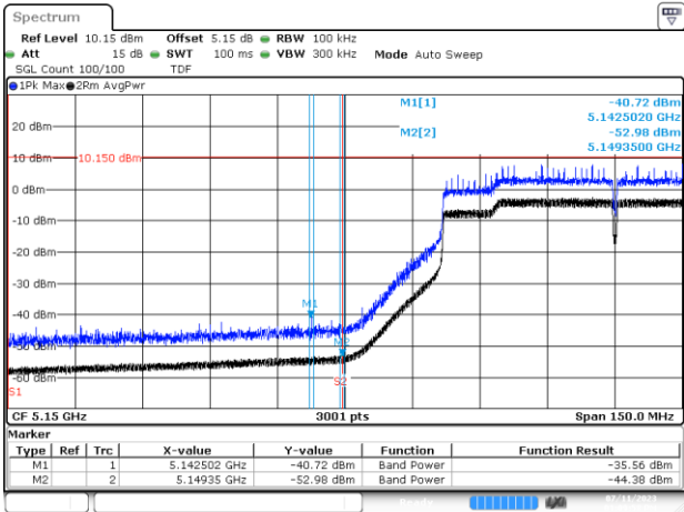
BE-R-LOW, MIMO-A, 802.11ac80-VHT8, Ch42
