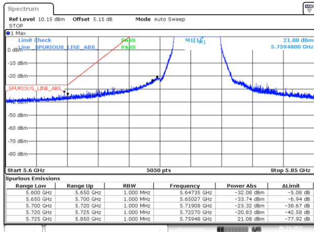
BE-NR-LOW, MIMO-B, 802.11n40-HT8, Ch151
