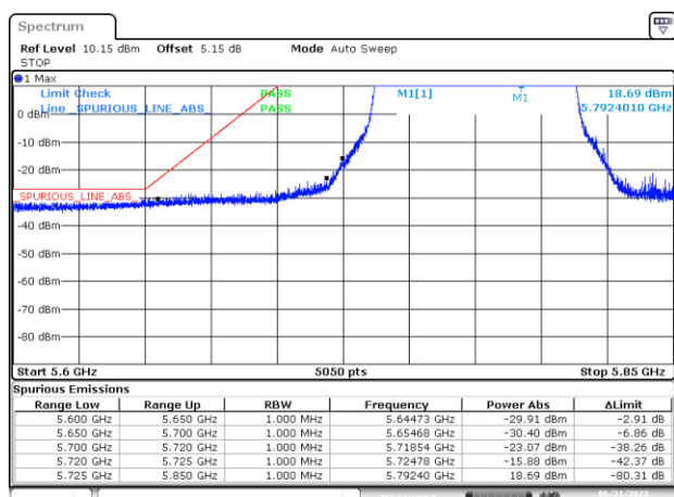
BE-NR-LOW, SISO-B, 802.11ac80-VHT0, Ch155
