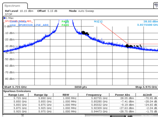
BE-NR-HIGH, SISO-B, 802.11ax/be20-MCS0, Ch165
