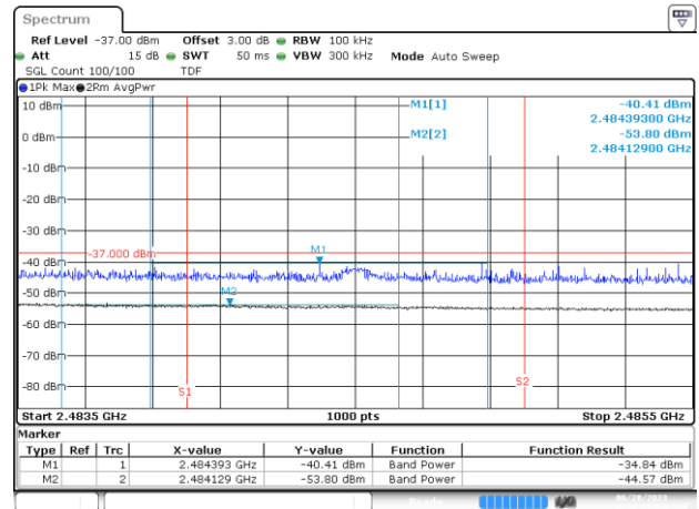
BE-R-HIGH-2MHz, MIMO-A, 802.11ax/be20-MCS0, Ch11
