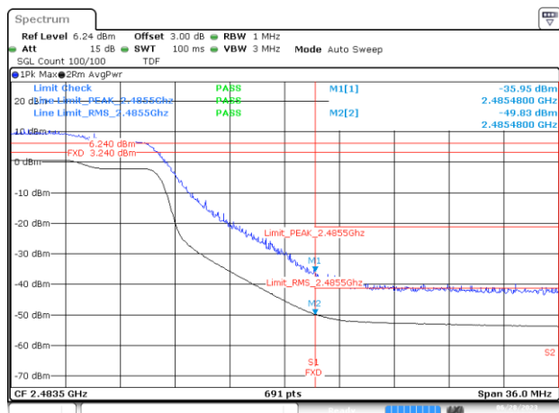
BE-R-HIGH, MIMO-A, 802.11n40-HT8, Ch10
