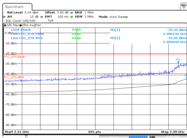
BE-R-LOW, MIMO-A, 802.11ax/be20-MCS0, Ch1
