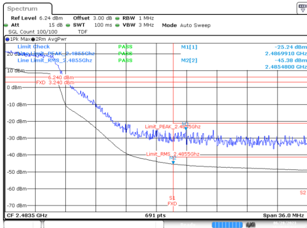
BE-R-HIGH, MIMO-A, 802.11ax/be20-MCS0, Ch11
