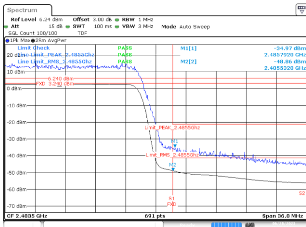
BE-R-HIGH, MIMO-A, 802.11ax/be20-MCS0, Ch13
