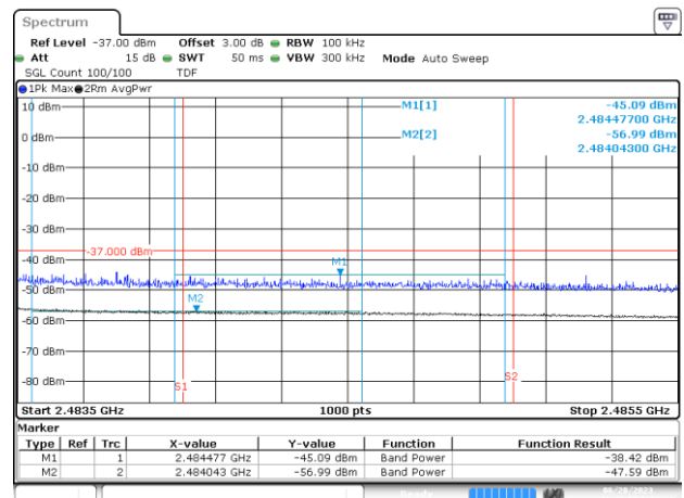
BE-R-HIGH-2MHz, MIMO-A, 802.11ax/be20-MCS0, Ch13
