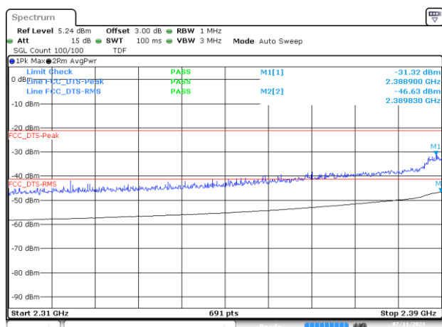
BE-R-LOW, MIMO-B, 802.11n20-HT8, Ch1
