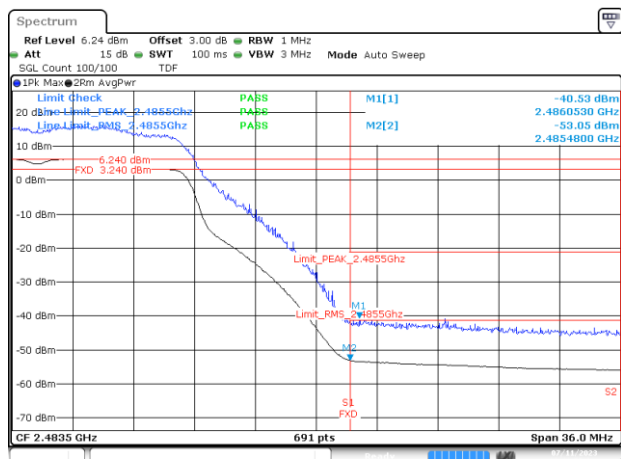
BE-R-HIGH, MIMO-B, 802.11n20-HT8, Ch12
