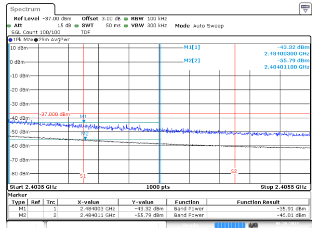
BE-R-HIGH-2MHz, MIMO-A, 802.11ax/be20-MCS0, Ch12
