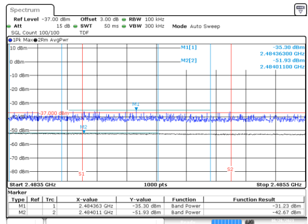
BE-R-HIGH-2MHz, SISO-A, 802.11ax/be20-MCS0, Ch11
