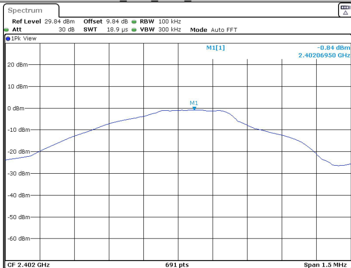
DH5_Ant1_2402_0~Reference
