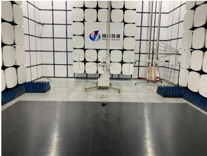
Radiated Emissions From 30MHz-1000MHz
