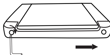
The running belt shifts to the left, tighten the left side
