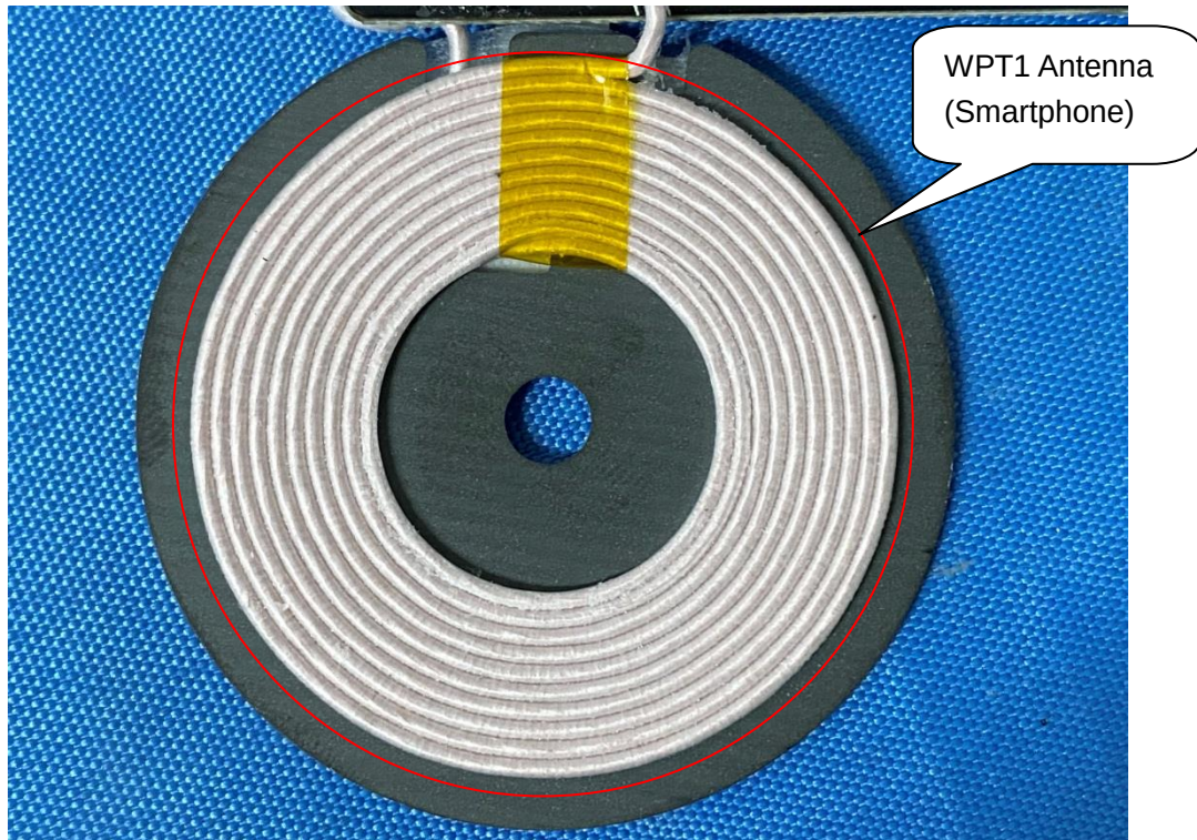
INTERNAL VIEW OF EUT (FIGURE 8)
