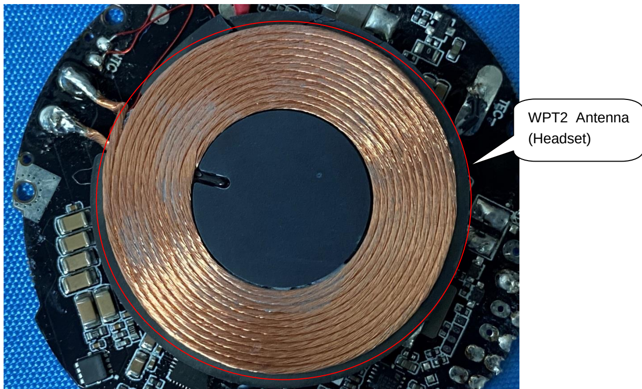
INTERNAL VIEW OF EUT (FIGURE 8)
