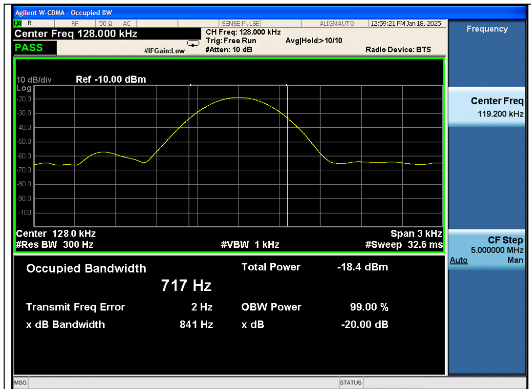
Test_Graph_ASK_Coil 2 nd _128kHz_-20dB Bandwidth
