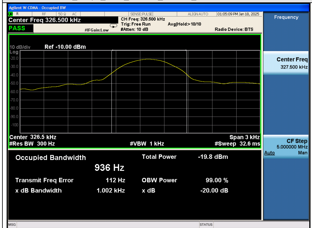
Test_Graph_ASK_Coil 3 rd _326.5kHz_-20dB Bandwidth
