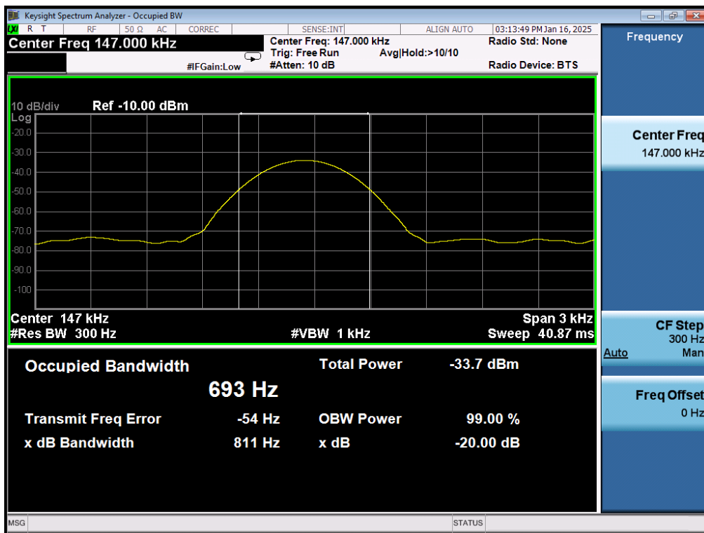
Test_Graph_ASK_Coil_147.0kHz_-20dB Bandwidth
