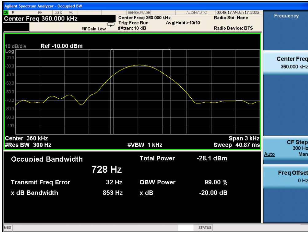
Test_Graph_ASK_Coil_360.0kHz_-20dB Bandwidth
