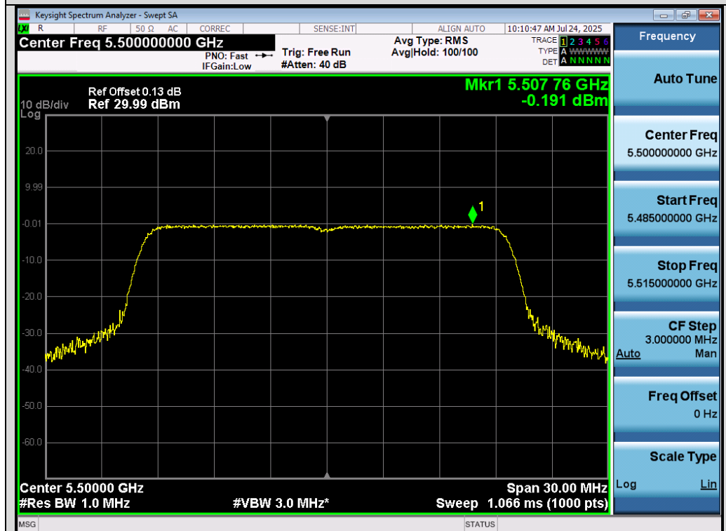
Test_Graph_802.11ax20_ANT1_5500_MCS0_PSD
