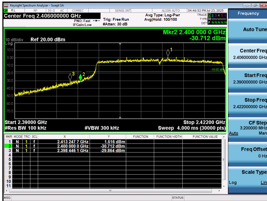
Test_Graph_802.11ax20_ANT1_2412_MCS0_Lower Band Edge Emissions
