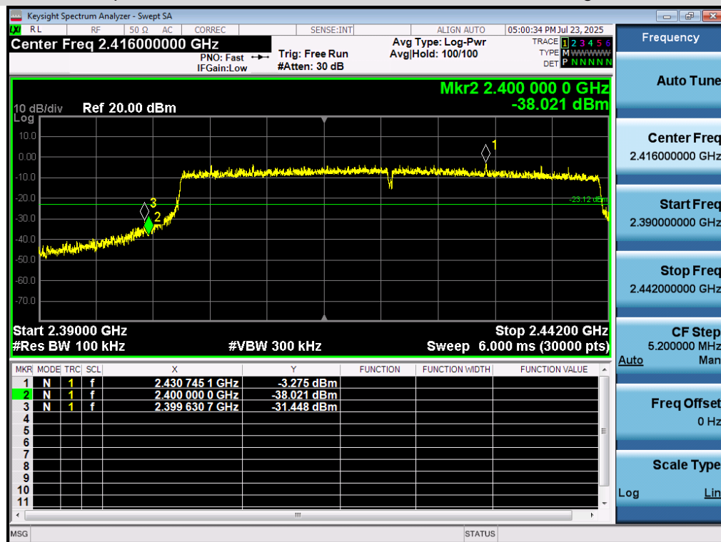
Test_Graph_802.11ax40_ANT1_2422_MCS0_Lower Band Edge Emissions
