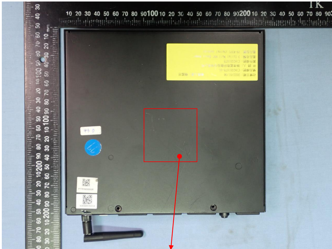
Label Placement Location (EUT Bottom View)
