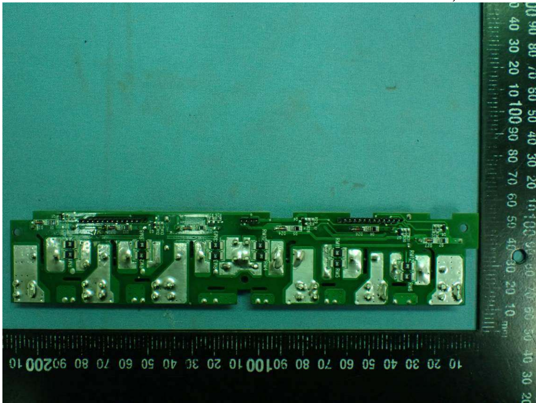
Figure 18 Internal Board, Back View
