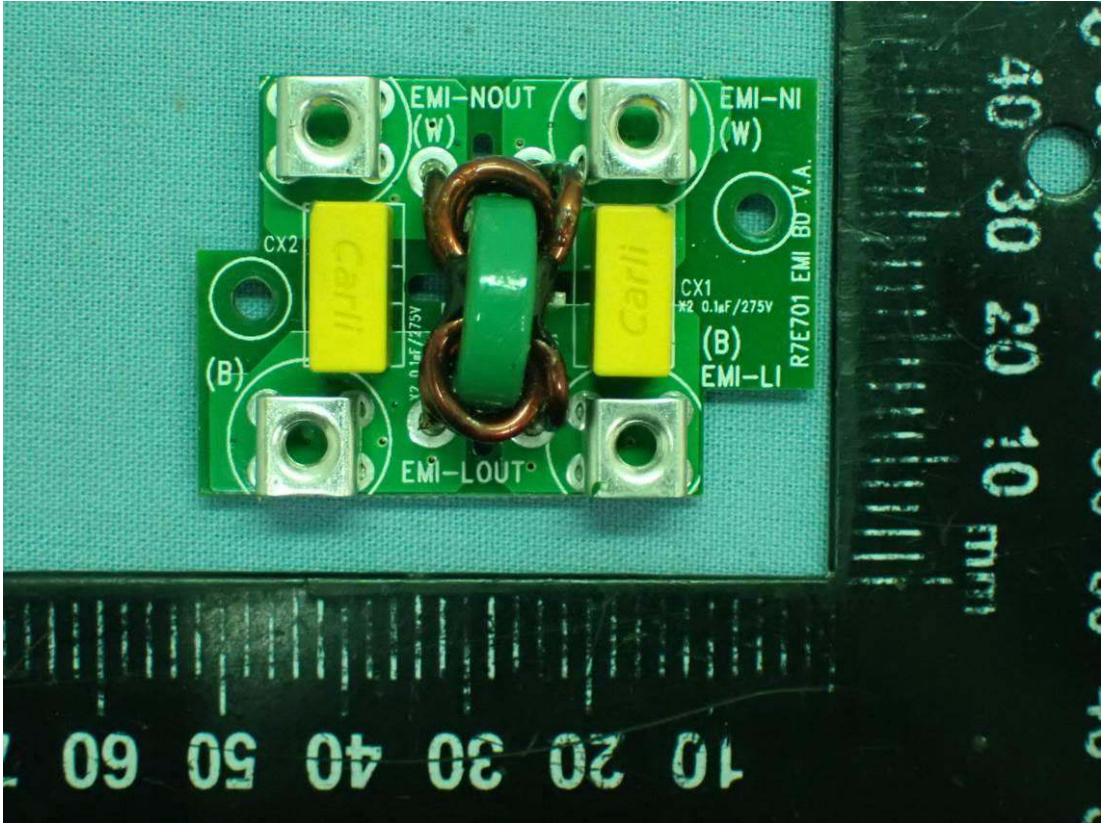
Figure 15 Internal Board, Front View
