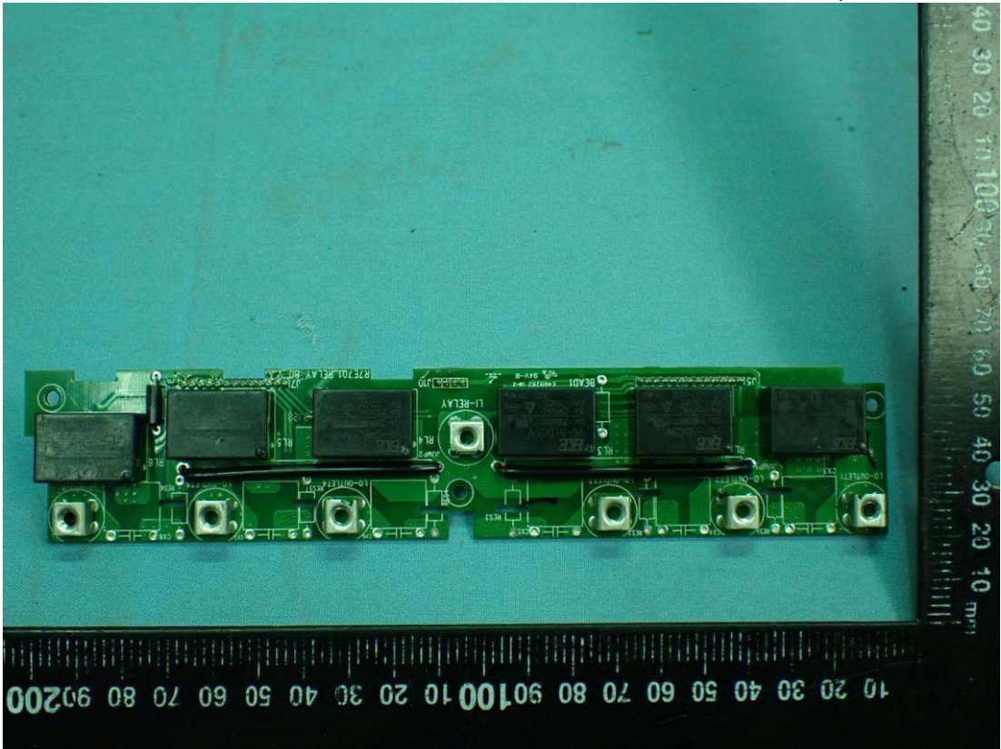
Figure 17 Internal Board, Front View
