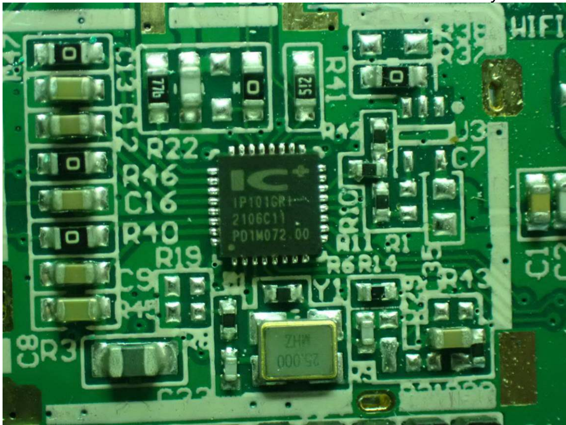
Figure 30 RJ45 Network IC & Crystal View
