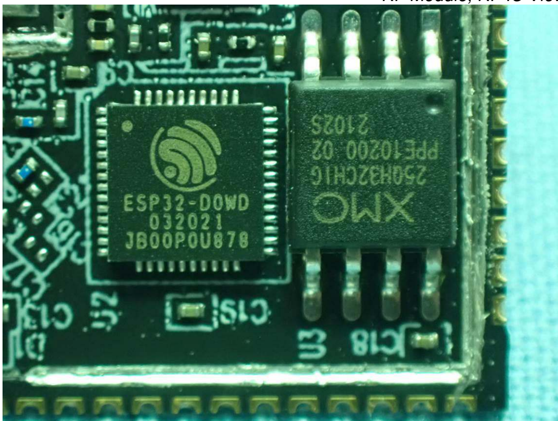
Figure 28 RF Module, RF IC View
