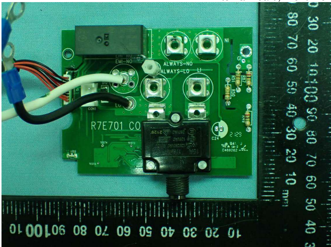
Figure 19 Internal Board, Front View
