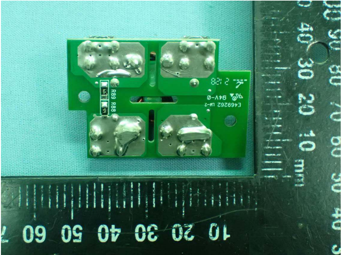
Figure 16 Internal Board, Back View
