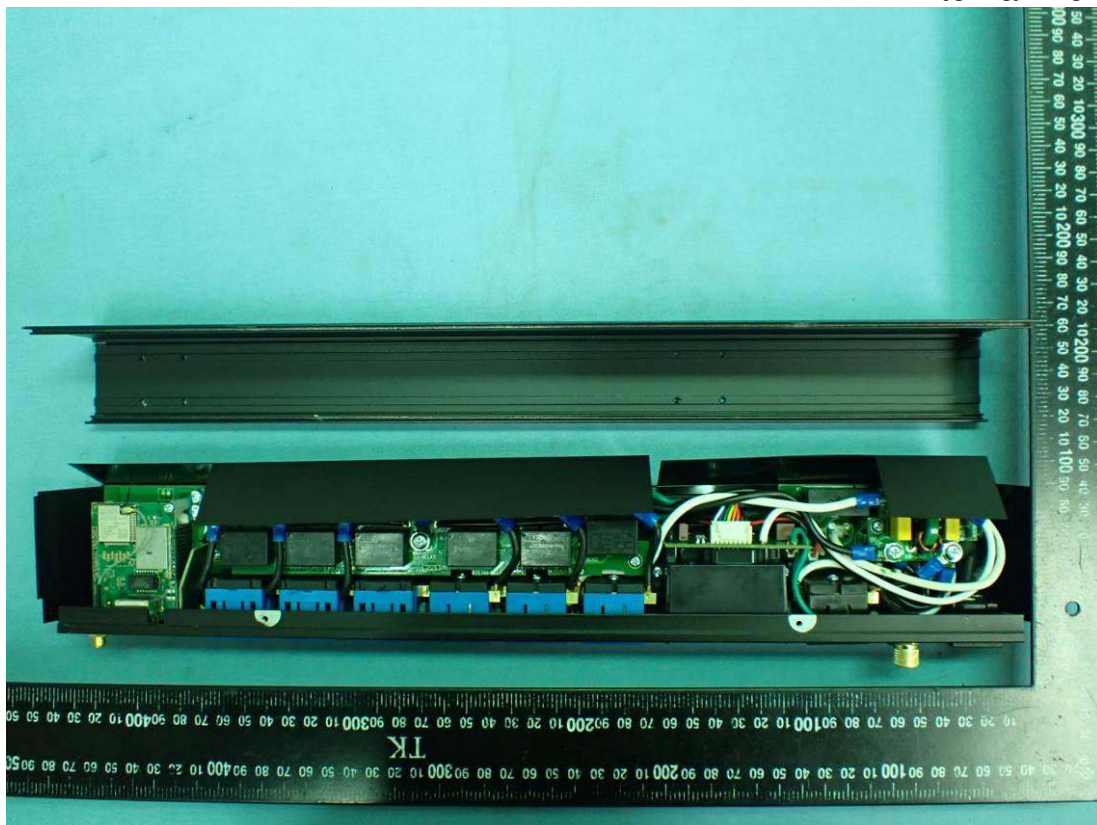
Figure 13 Internal View
