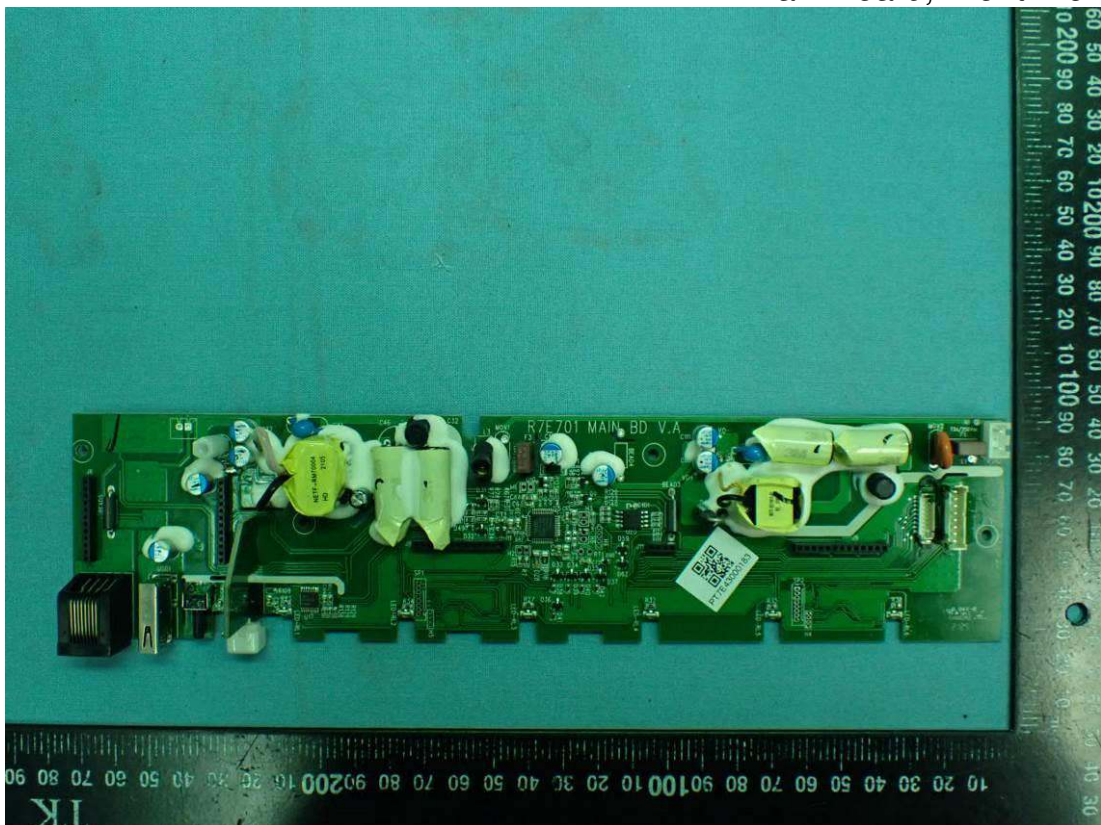
Figure 21 Main Board, Front View
