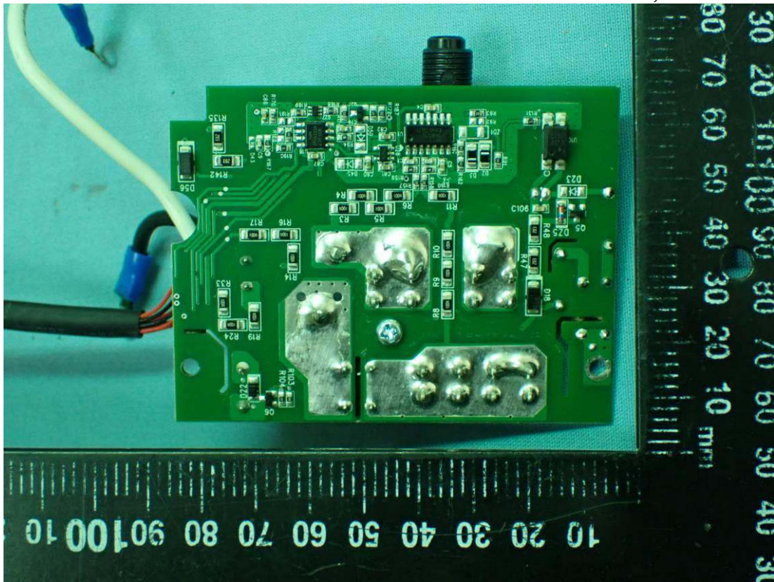
Figure 20 Internal Board, Back View
