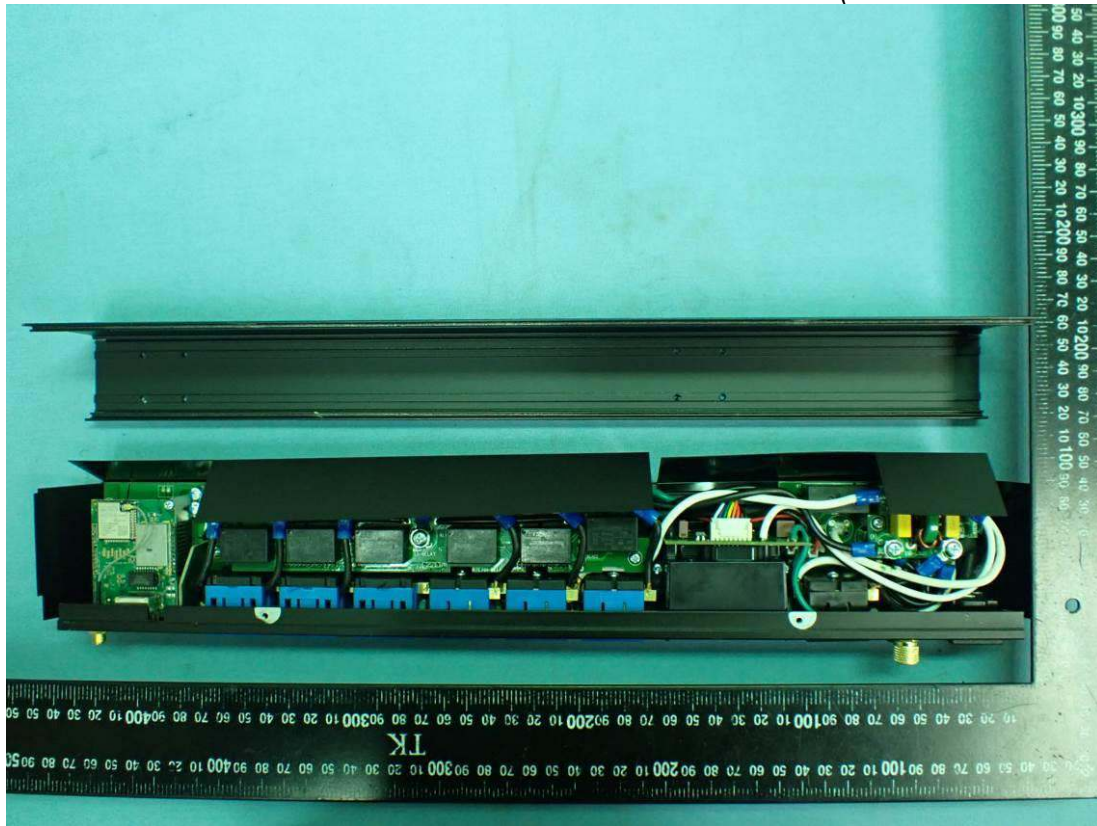
Figure 12 Internal View (Removed Cover)
