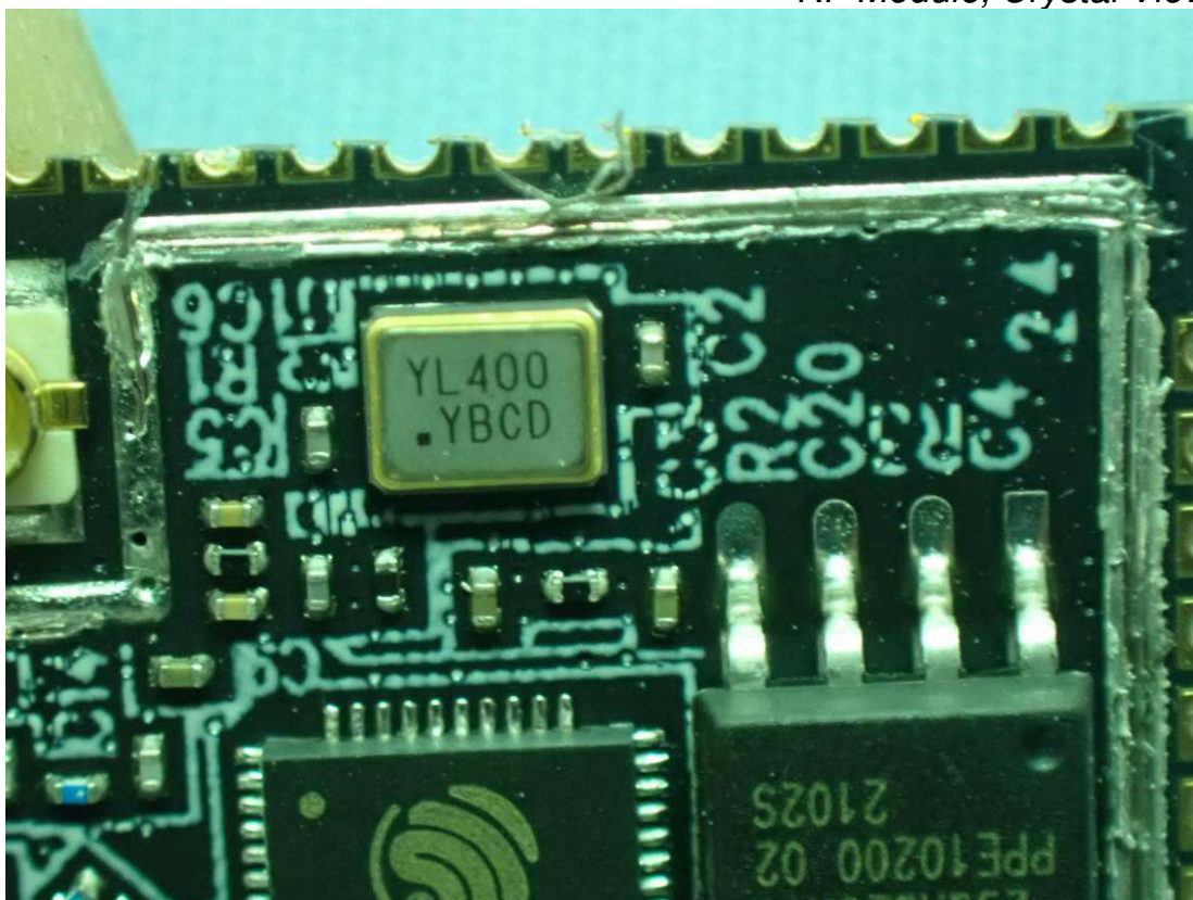
Figure 29 RF Module, Crystal View
