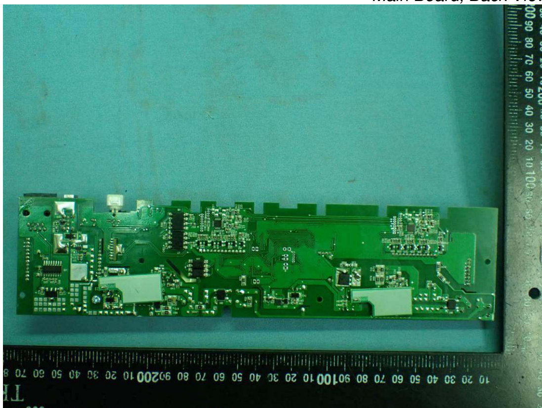
Figure 22 Main Board, Back View
