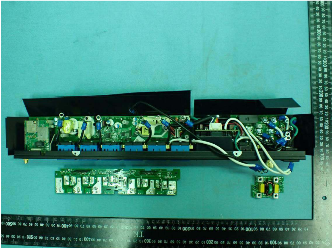
Figure 14 Internal View
