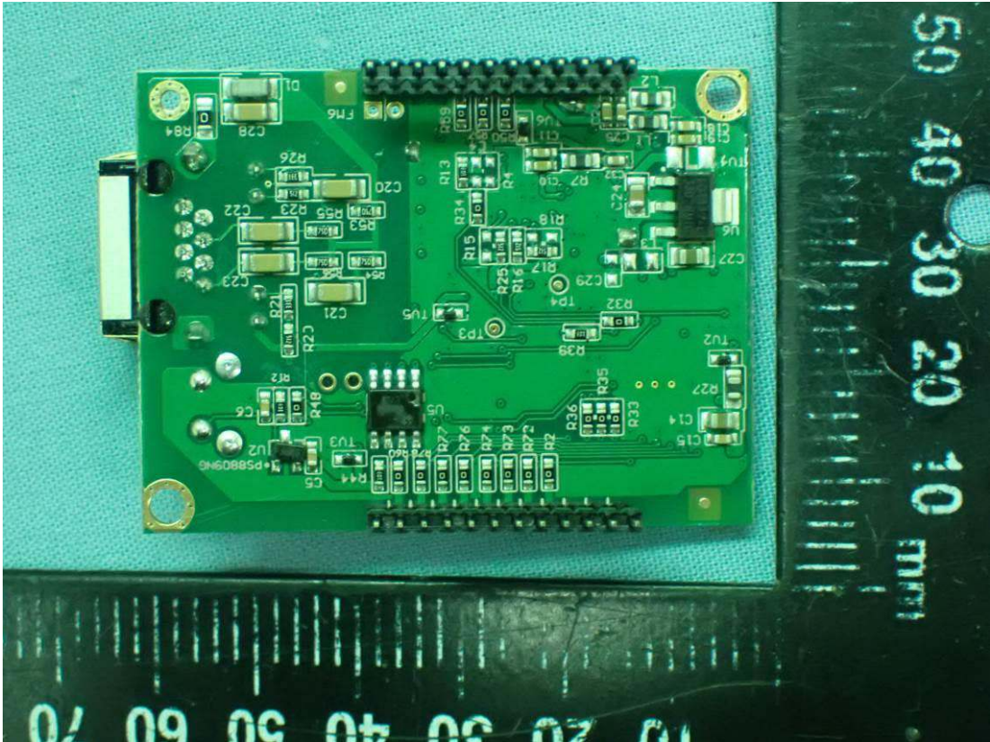
Figure 24 Internal Board, Back View
