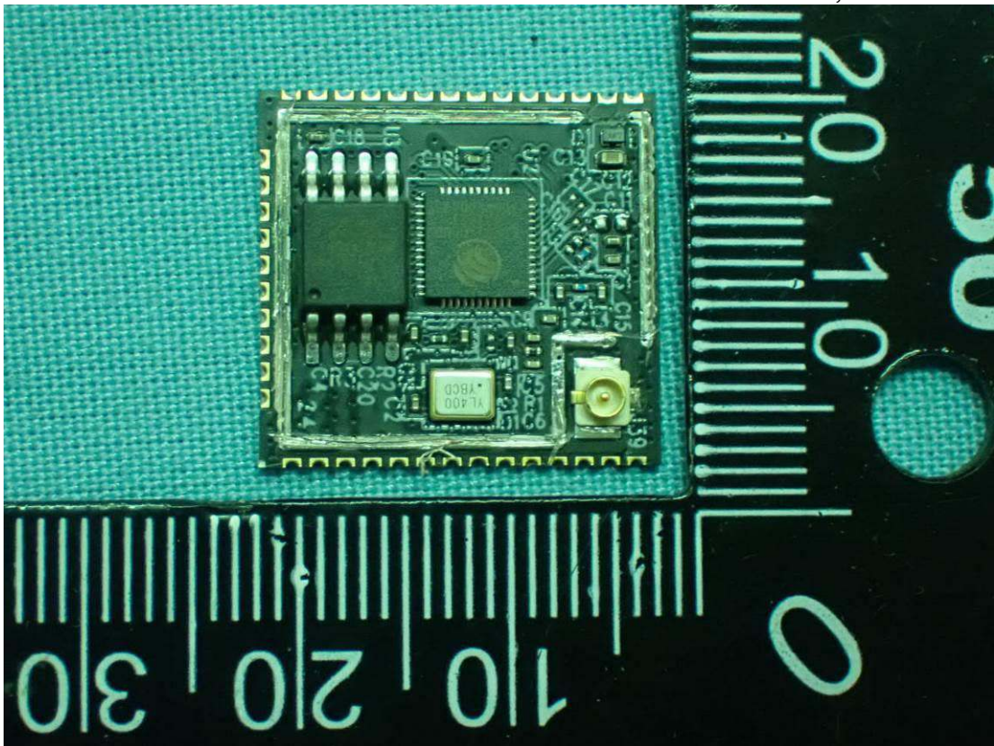
Figure 26 RF Module, Front View
