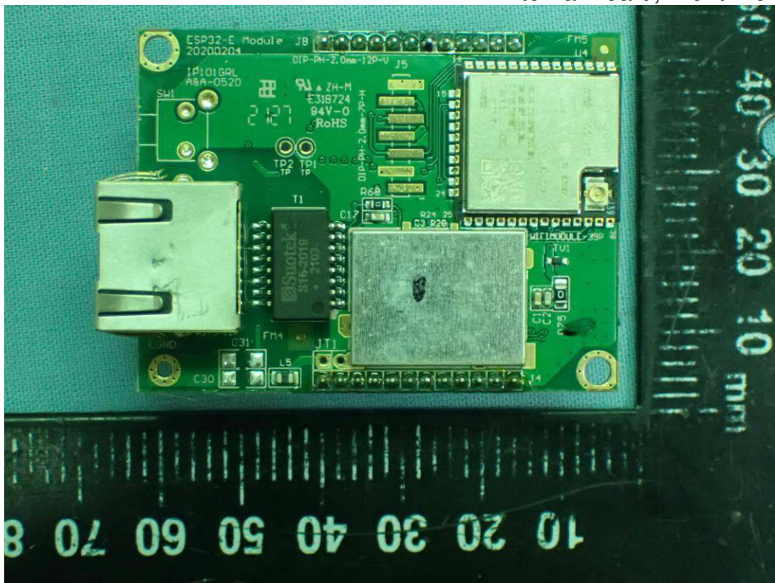
Figure 23 Internal Board, Front View
