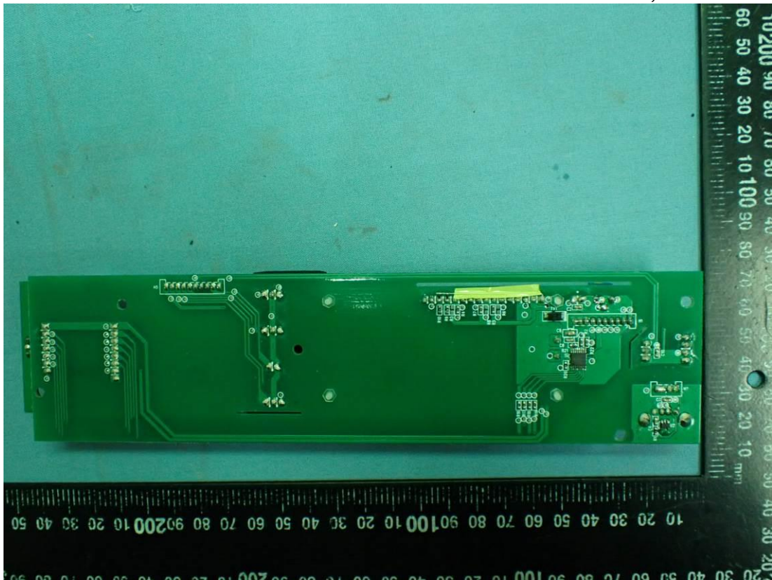
Figure 22 Internal Board, Back View
