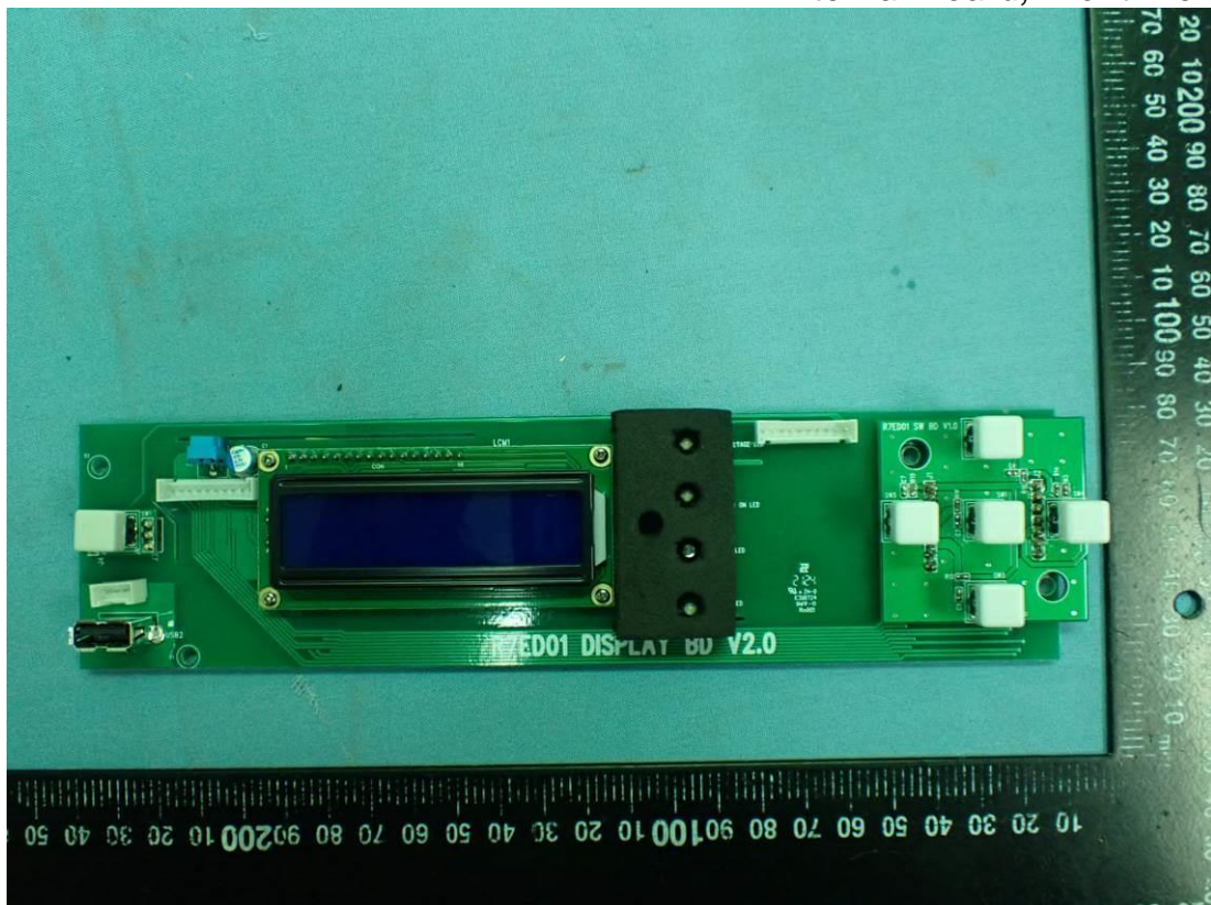
Figure 21 Internal Board, Front View
