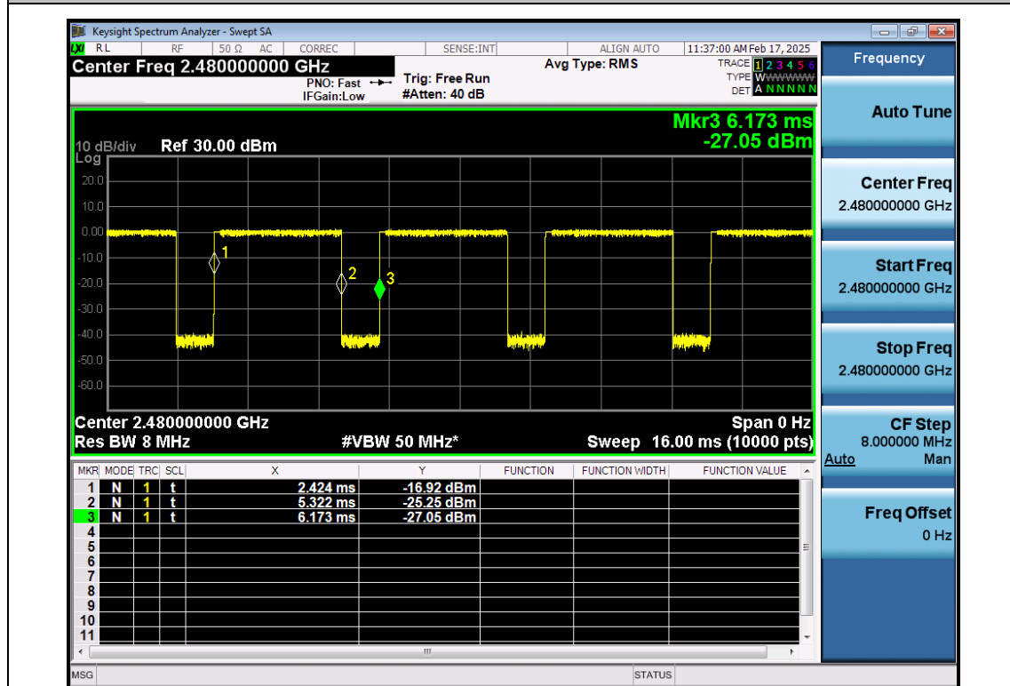
EDR-π /4-DQPSK-Ant1-2480
