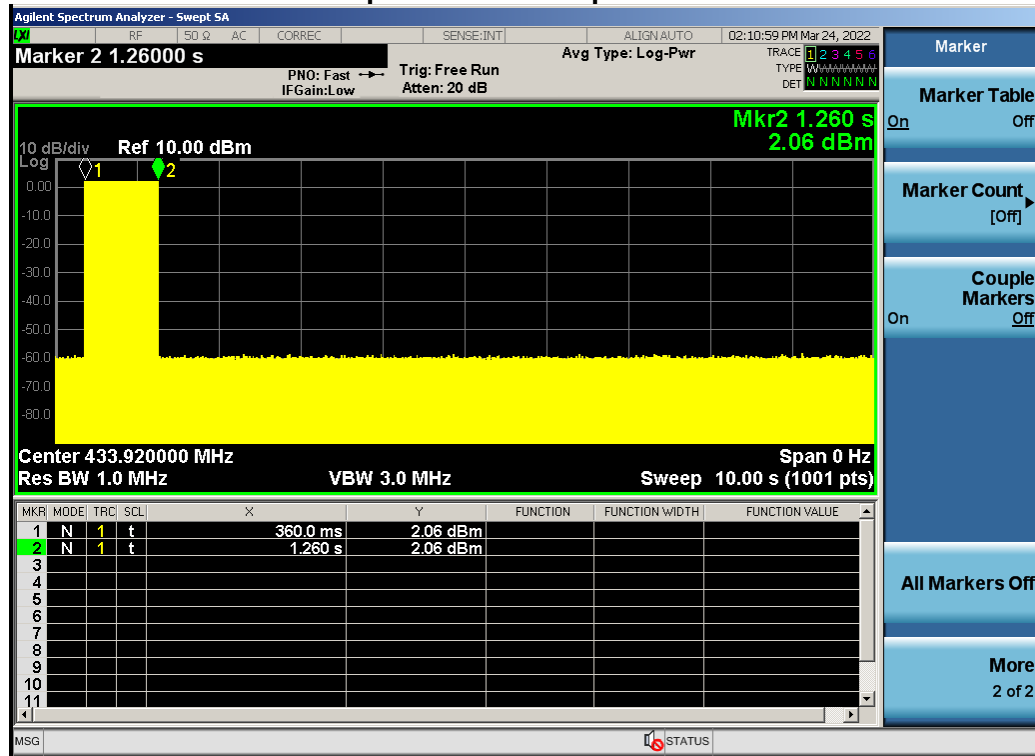
Test Graphs Of Launch Operation Time
