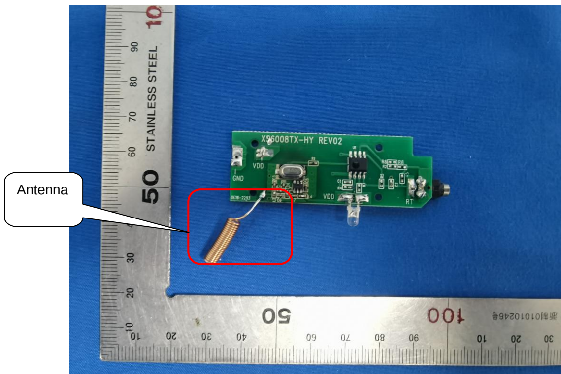
INTERNAL VIEW OF EUT (FIGURE 2)
