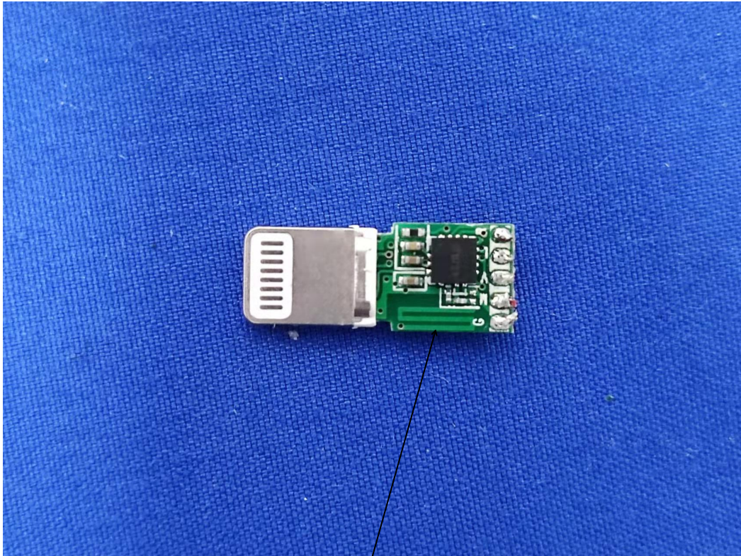
PCB ANTENNA
