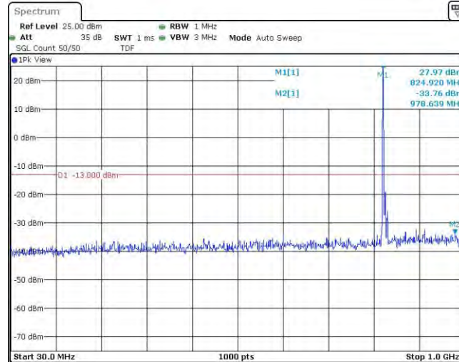
Band5-5MHz-QPSK-20425-1RB#0-Range2:1000~10000MHz
