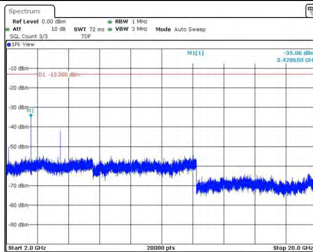
Band4-3MHz-16QAM-20175-1RB#0-Range1:30~1000MHz
