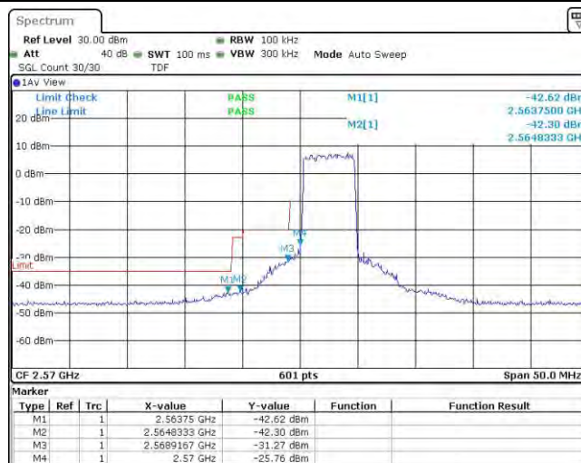
Band38-5MHz-16QAM-37775-25RB#0
