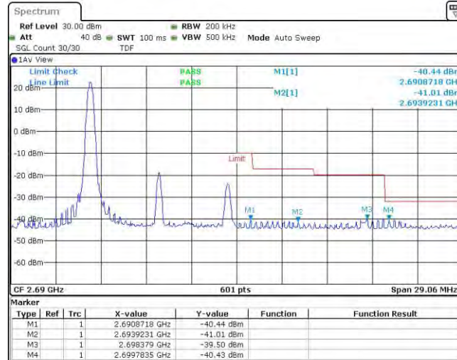
Band41-10MHz-QPSK-41540-1RB#49
