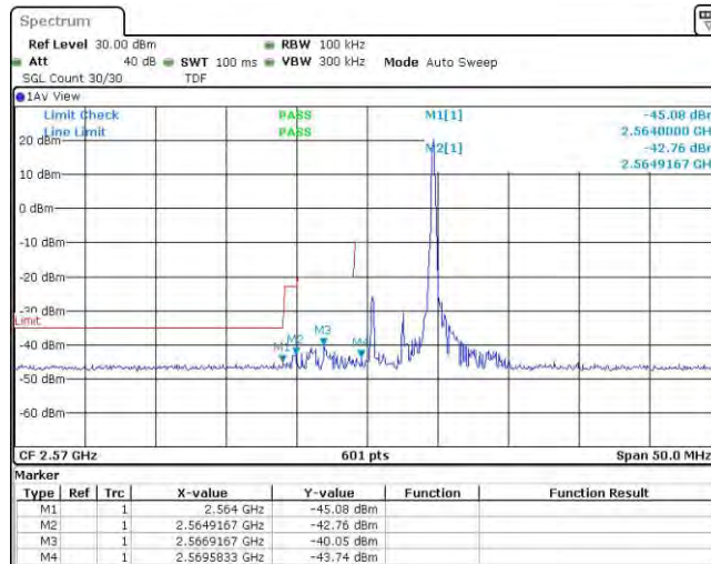
Band38-5MHz-16QAM-37775-25RB#0
