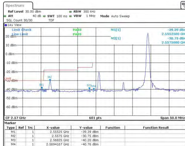
Band38-15MHz-QPSK-37825-75RB#0
