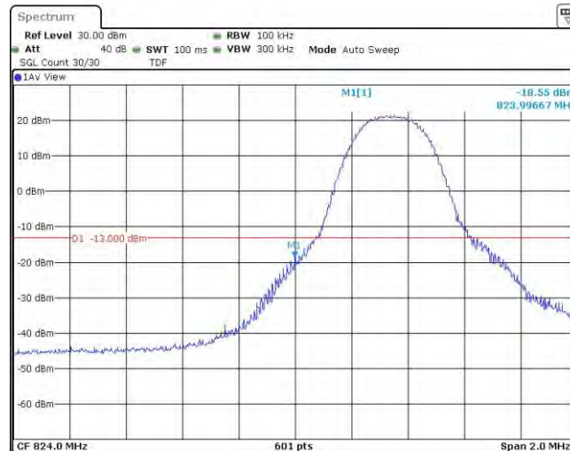
Band5-5MHz-QPSK-20425-1RB#24
