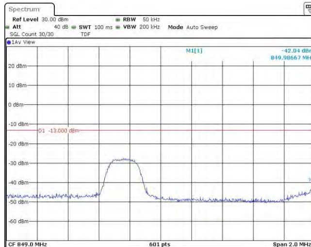
Band26-3MHz-QPSK-27025-1RB#14
