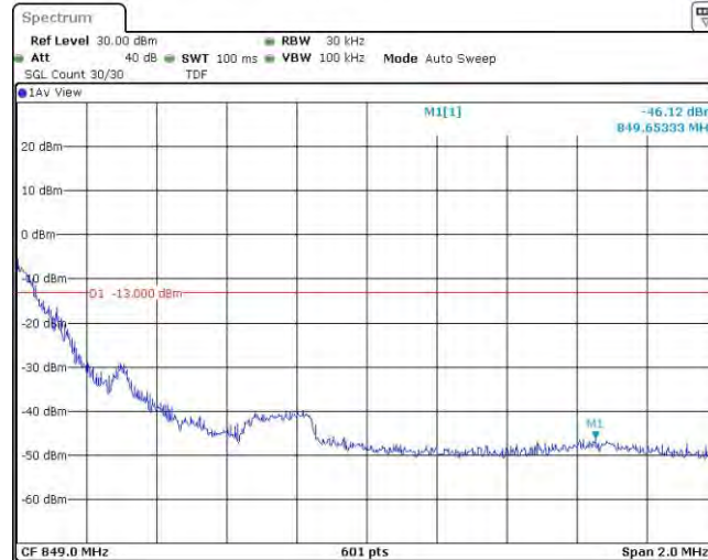
Band5-1.4MHz-16QAM-20643-1RB#5
