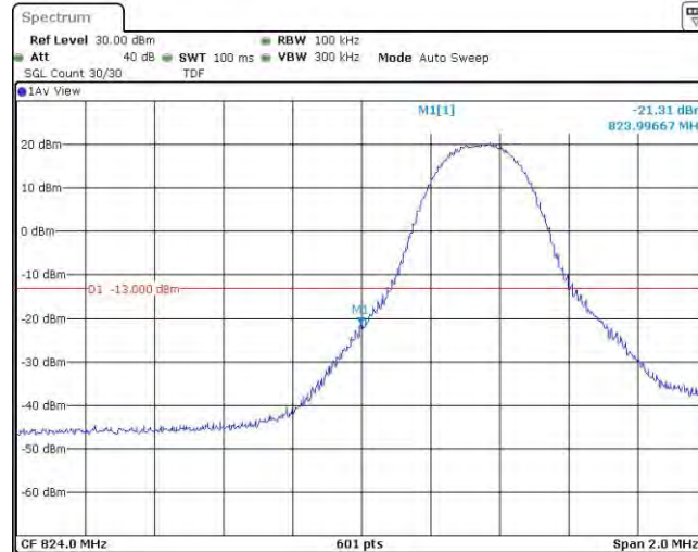
Band5-5MHz-16QAM-20425-1RB#24
