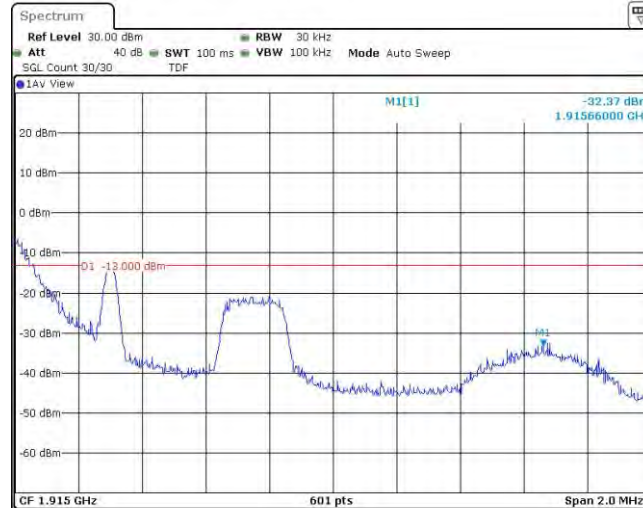
Band25-1.4MHz-16QAM-26683-1RB#5
