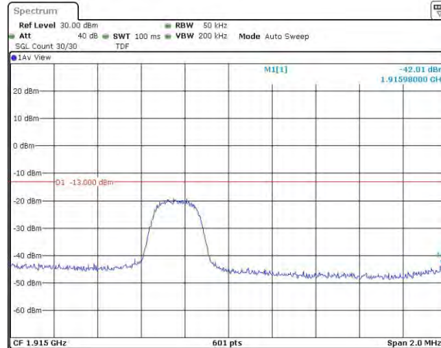
Band25-3MHz-16QAM-26675-1RB#14
