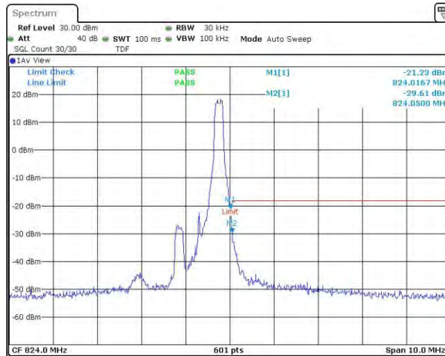
Band26-1.4MHz-QPSK-26783-6RB#0
