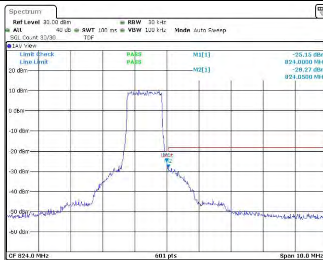
Band26-1.4MHz-QPSK-26797-1RB#0
