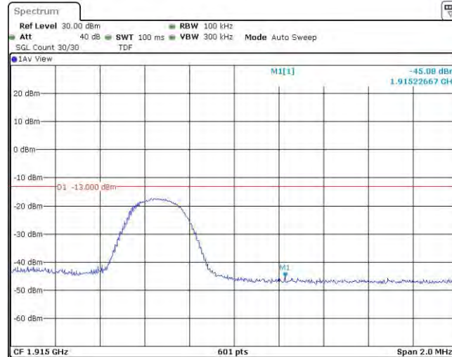
Band25-5MHz-QPSK-26665-1RB#24
