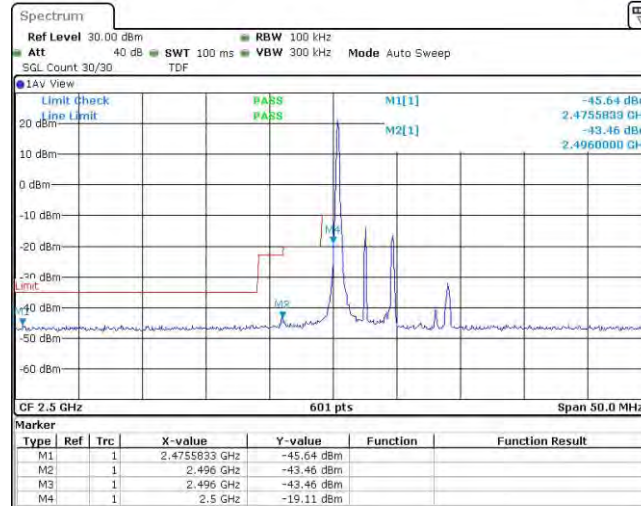
Band7-5MHz-16QAM-20775-1RB#24
