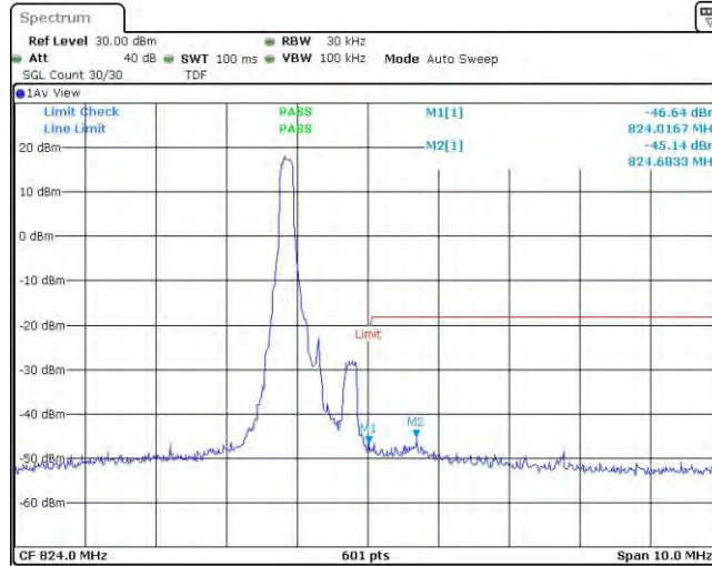
Band26-1.4MHz-QPSK-26783-1RB#5
