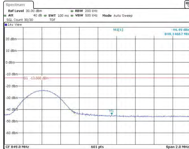
Band5-10MHz-16QAM-20600-1RB#49
