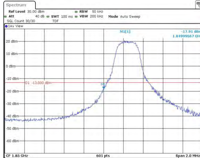
Band25-3MHz-16QAM-26055-1RB#14
